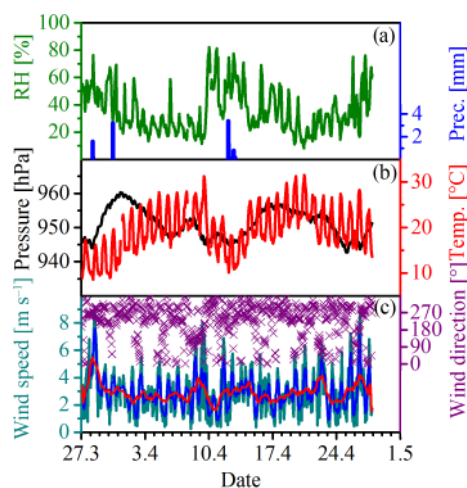
Figure 2. One-hour averages of meteorological parameters (a) relative humidity (green) and precipitation (blue); (b) unreduced pressure (black) and temperature (red); (c) wind direction (purple crosses) and speed (cyan) and its running means of 6 h (blue) and 24 h (red) during the campaign measured at CAO by the Department of Labour Inspection of Cyprus (DLI).
