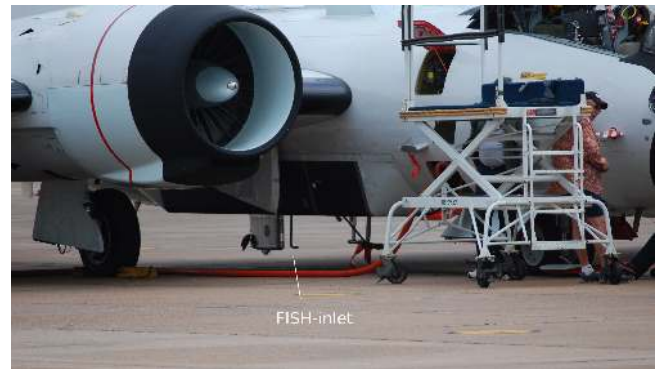
Figure 6. Bottom-mounted FISH inlet at WB-57 (photo: Armin Afchine).
