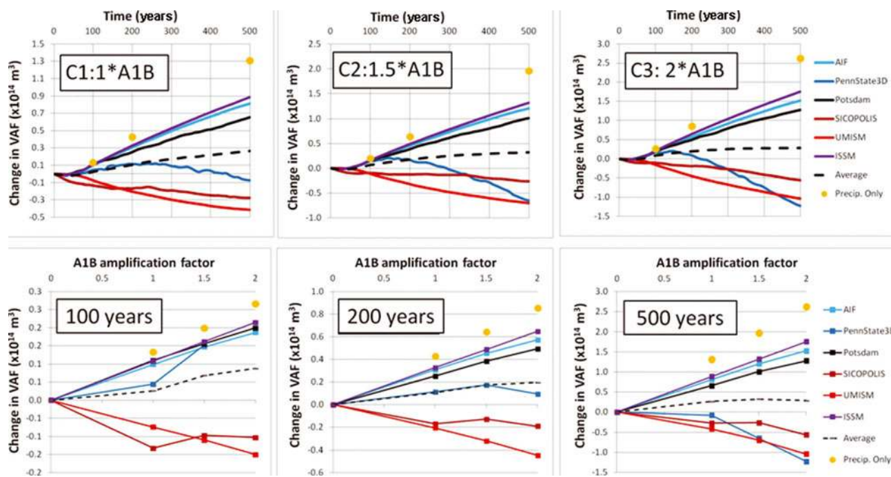
Fig. 9. Change of VAF for the climate sensitivity experiments of the Antarctic ice sheet. Upper panels show calculated VAF change for the triplet of cases where prescribed temperature and precipitation changes are taken from the A1B scenarios of the IPCC AR4: left, C1, 100% of A1B changes applied; middle, C2, 150% of A1B changes applied; right, C3, 200% of A1B changes applied. Lower panels illustrate the sensitivity of VAF change for the same experiments vs the amplification of the applied climate changes at 100, 200 and 500 years after the simulation start. Orange circles indicate the VAF change resulting only from the applied change in precipitation at 100, 200 and 500 years. See Table 2 and Appendix A for descriptions of the various models.
