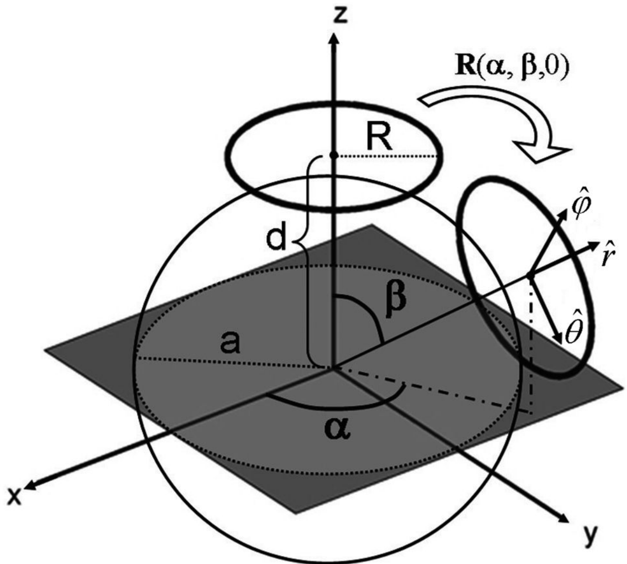
Fig. 1. Schematic representation of the spherical sample geometry, with two exemplary loop coils arranged on a spherical surface at distance \sqrt{a^2 + R^2} from the center of the sphere. SNR and SAR calculations were performed on a transverse plane through the center of the object.
