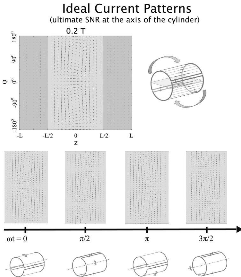
Fig. 7. Ideal surface current patterns associated with the best possible SNR at a voxel on the axis of a cylindrical sample at 0.2 T. On the left-hand side of the top row, current patterns are plotted for an arbitrary time point on a two-dimensional “unwrapped” view of the cylindrical surface (with the axial and azimuthal coordinates on the horizontal and vertical axis, respectively), whereas on the right-hand side, a schematic representation shows how the current patterns evolve in time. In the middle and bottom rows, the current patterns are shown together with explanatory diagrams for four time points. Ideal currents patterns, which resemble the rotating dual distributed-loop pattern seen in a sphere (Figure 3), may also be recognized as a distributed birdcage-like pattern, in which z -directed “rung” currents vary sinusoidally around the circumference of the cylinder, connected by encircling “end-ring” return currents. The entire current pattern precesses at the Larmor frequency around the axis of the cylinder (i.e. the z -axis).
