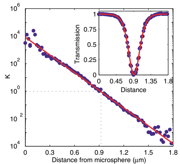
FIG. 3 (color online). Coupling parameter K vs taper-sphere separation for a 65- \mu\text{m} -diameter microsphere. The data show a linear relation between \ln K and x , with a least squares fit (solid line). Ideality inferred at contact is greater than 99.99%. The dotted line marks the critical coupling point ( K = 1 at x = 0.91 \mu\text{m} ). The inset shows transmission vs position data.
