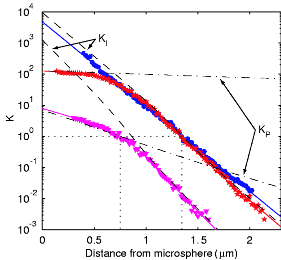
FIG. 2 (color online). K vs position for various taper diameters for a 67- \mu\text{m} -diameter microsphere. The data represent taper diameters of approximately 1.2 \mu\text{m} (circles), 1.35 \mu\text{m} (stars), and 1.65 \mu\text{m} (triangles). Solid curves are fits using Eq. (6). The ideality at contact in the data (extrapolating fits to zero gap) is > 99.98\% , 99%, and 88%, respectively. Data show that for increased taper diameter higher-order-mode coupling causes a deviation from the ideal case (dashed line). The dash-dotted line represents K_P , which is related to ideality through Eq. (5). Dotted lines mark the critical coupling point.
