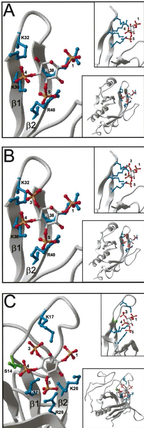
Fig. 7. Theoretical model for interaction between BTK and Ins(1,3,4,5)P 4 . Ribbon diagrams are shown with certain key residues highlighted as ball and stick models as indicated. Lysine and arginine residues are in blue, and serine is green. (A) The solved crystal structure of the PH domain of PLC \delta complexed with Ins(1,4,5)P 3 . (B) Theoretical model for interaction between PLC \delta complexed with Ins(1,3,4,5)P 4 . Note that the lysine (K32) in the first position of the \beta 1– \beta 2 loop is in position to block access of the 3-phosphate in Ins(1,3,4,5)P 4 to the binding site. (C) Diagram depicting a theoretical model for the interaction between the PH domain of BTK and Ins(1,3,4,5)P 4 . In contrast to K32 of PLC \delta , the serine (S14) in the first position of the \beta 1– \beta 2 loop allows access of the 3-phosphate in Ins(1,3,4,5)P 4 to this binding site. In addition, lysine at position 17 in the \beta 1– \beta 2 loop is in position to contact the 3-phosphate of Ins(1,3,4,5)P 4 to stabilize the interaction. The model is based on the BTK PH domain crystal structure coordinates but has been modified by replacing C28 with R and energy minimizing the \beta 1– \beta 2 loop in the presence of Ins(1,3,4,5)P 4 ligand as described in Materials and methods. The structure of the BTK PH domain has been energy minimized in the presence of ligand between residues 13–25. Three views for each structure are shown: the larger structure is face on; the upper inset is the same structure rotated counterclockwise on the y-axis 55°; the lower inset is the face on view of the complete PH domain to provide orientation. Ligand atoms are colored as follows: carbon, white; oxygen, red; phosphorous, orange.
