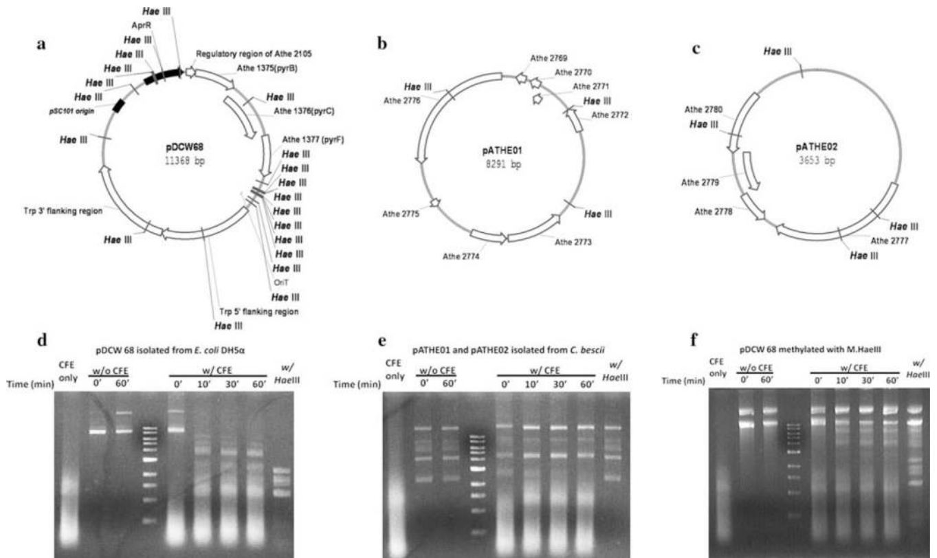
Fig. 1. Detection of a HaeIII-like restriction/modification system in C. bescii . a pDCW68; b pATHE01; c pATHE02; d pDCW68 isolated from E. coli DH5 \alpha incubated with CFE from C. bescii ; e pATHE01 and pATHE02 isolated from C. bescii incubated with CFE from C. bescii ; f pDCW68 isolated from E. coli treated with M.HaeIII and incubated with CFE from C. bescii . Features originating from E. coli are shaded in black , and features from C. bescii in white ; Apr R , apramycin resistant gene cassette; Trp, Athe 2105-tryptophan synthetase \alpha subunit; OriT , origin of transfer for conjugation; pSC101, low copy replication origin in E. coli ; HaeIII restriction sites are indicated. All incubation times were as indicated
