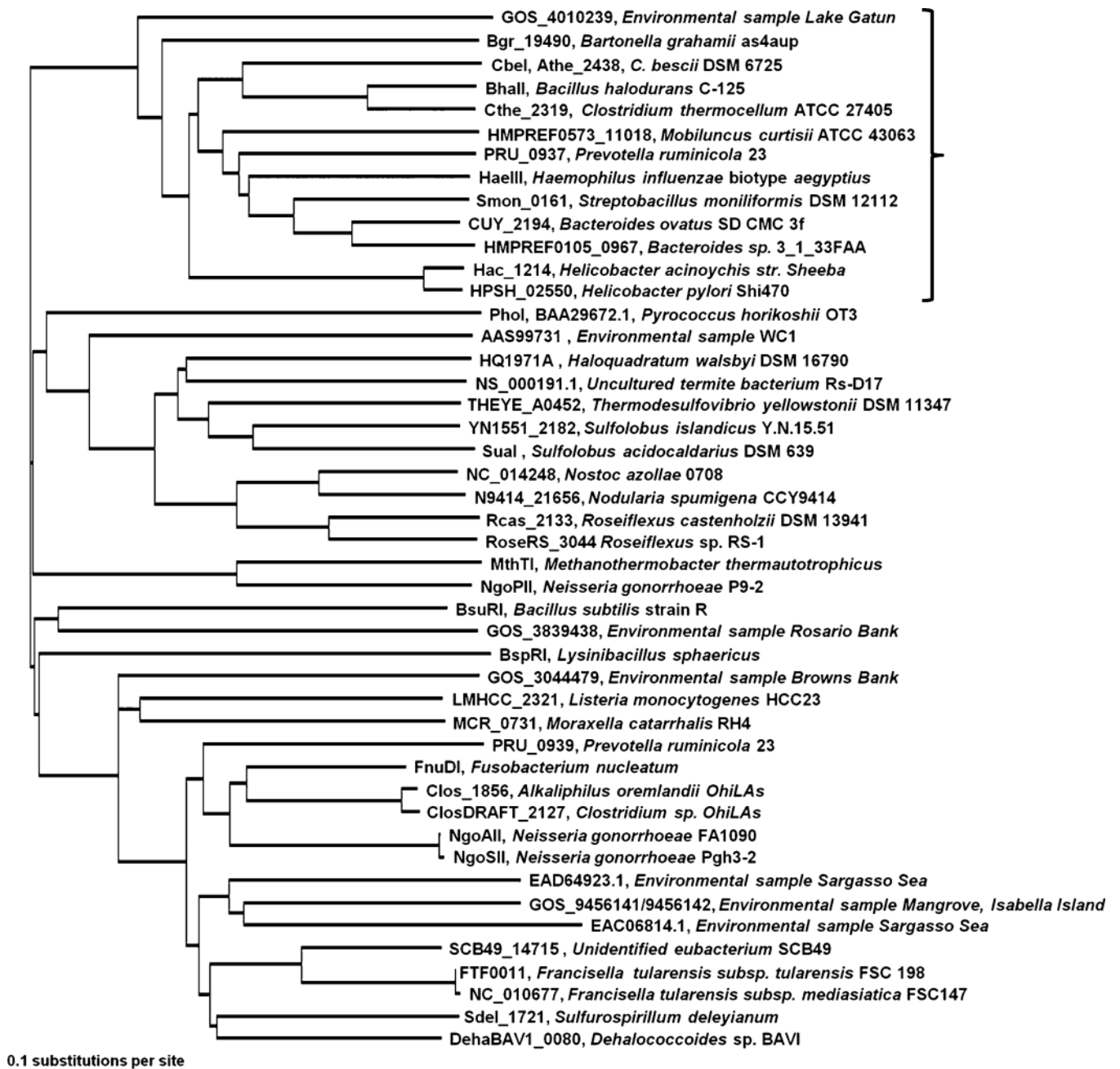
Fig. 4. Phylogram alignment of 46 HaeIII-like restriction enzymes. The host organism for each restriction enzyme is indicated as well as the protein name, when available; otherwise, the GenBank locus tag or accession number is given. The distance scale is indicated by a bar defining the distance for 0.1 amino acid substitution per site. The bracketed organisms represent those containing this new subfamily of HaeIII-like enzymes that includes CbeI
