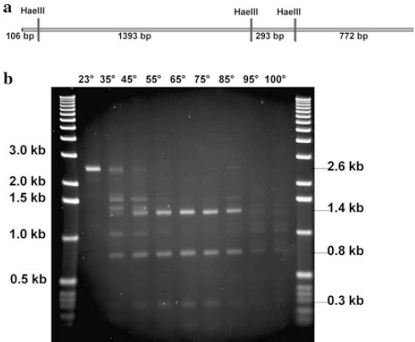
Fig. 3. Temperature profile of purified CbeI endonuclease activity. a The 2.558-kb DNA substrate synthesized as described in the “Materials and methods.” HaeIII cleavage sites are marked by vertical lines , and predicted cleavage fragment sizes are indicated below the line . b pDCW72 used for His-tagged expression of CbeI. The substrate was incubated for 10 min with 0.5 ng protein at the temperatures indicated, and the cleavage products were separated on 1.2% agarose gel. The position of the full-length undigested fragment and the three major cleavage products derived by digestion with CbeI are indicated by arrows
