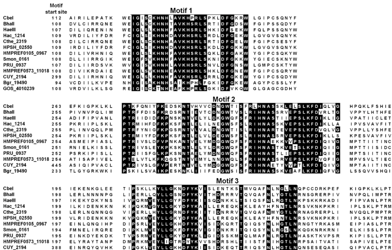
Fig. 5. Amino acid sequence alignment of CbeI with the subgroup identified in Fig. 4. Amino acid identity is shown as shaded areas with the position of the motif within the protein sequence. Motif start site is indicated. Motif 1: 7.0e-220, motif 2 1.9e-278, motif 3 1.6e-185
