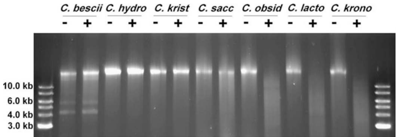
Fig. 6. Distribution of HaeIII-like restriction/modification systems in Caldicellulosiruptor species. Total DNA isolated from seven different species were incubated (–) without or (+) with commercially available HaeIII endonuclease at 37°C for 1 h according to the manufacturer’s instructions (NEB). C. bescii ; C. hydro , C. hydrothermalis ; C. krist , C. kristjansonii ; C. sacc , C. saccharolyticus ; C. obsid , C. obsidiansis ; C. lacto , C. lactoaceticus ; C. krono , C. kronotskyensis . Also visible in the C. bescii lanes are the undigested native plasmids from that strain, pATHE01 (8.3 kb) and pATHE02 (3.6 kb)
