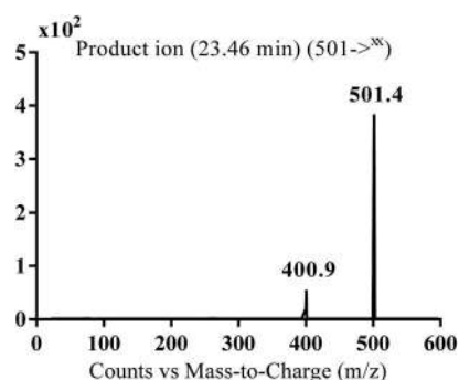
Fig. 10 MS 2 mass spectra of MA501 molecular ion peaks at m/z 501.
