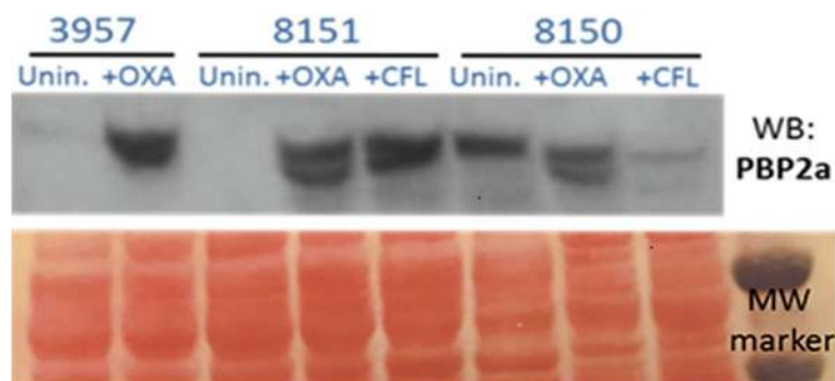
Fig. 1 Western blot analysis of PBP2a protein in lysates of MRSP strains grown without and with subinhibitory concentrations of oxacillin (OXA) and cephalixin (CFL) at 0.5 µg/ml. Lower image correspond to Ponceau staining used as loading control. Oxacillin (OXA), cephalixin (CFL), uninduced (Unin)
