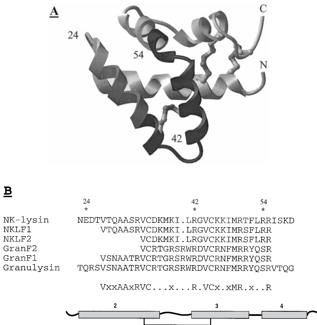
Figure 1 Solution structure of NK-lysin and primary structures of synthetic peptides
