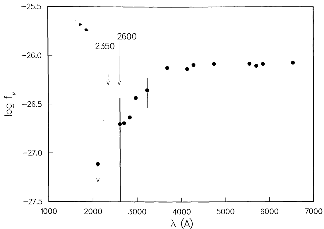
Fig. 1. Continuum spectral energy distribution of 0237 – 233.
