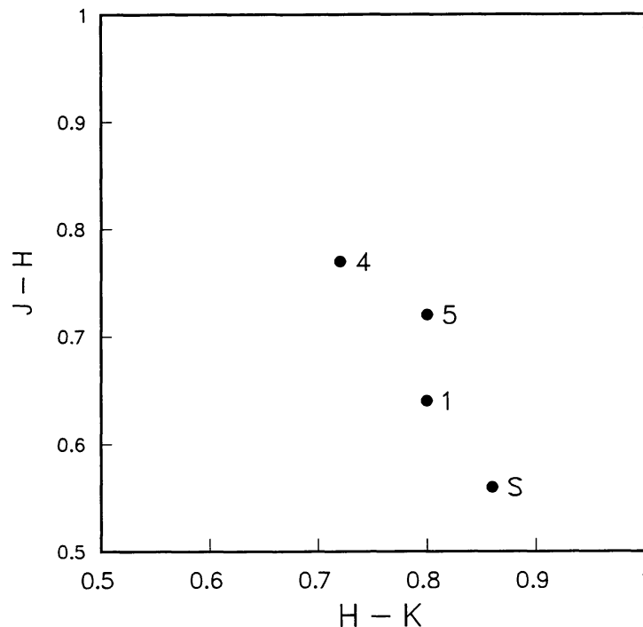
Fig. 4. The (J-H) versus (H-K) diagram for 3 quasars and \nu Sgr. Symbols have the same meaning as in Figure 2.
