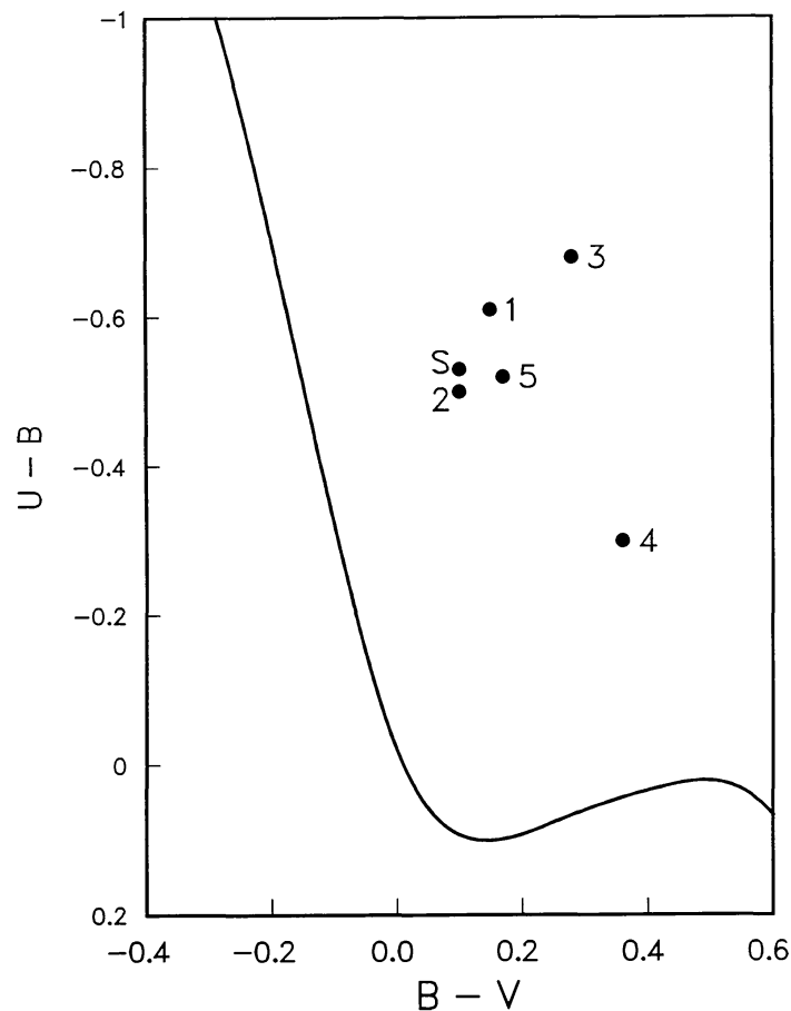
Fig. 2. (U-B) versus (B-V) plot. Key to points 1: 0237-233, 2: 0851+197, 3: 1225+317, 4: 1246-057, 5: 1448-232, S: \nu Sgr.
