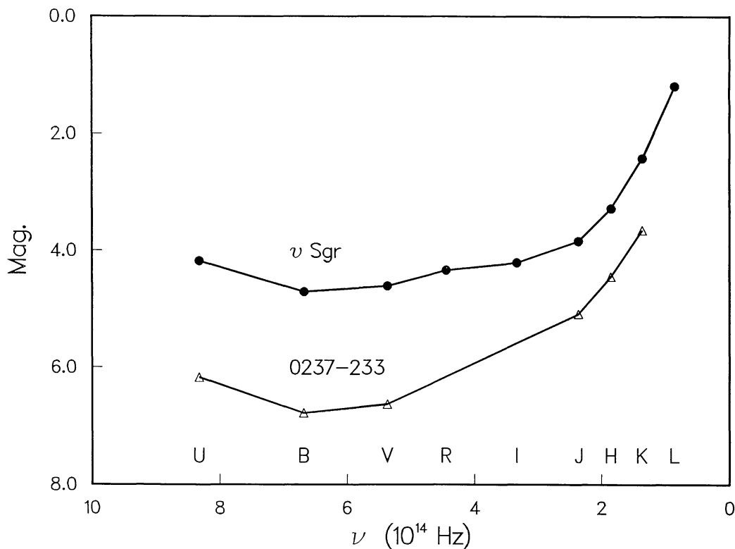
Fig. 3. The colours of \nu Sgr and 0237 – 233. The data points for \nu Sgr are from Lee and Narai (1967) and those for 0237 – 233, from Hewitt and Burbidge (1987) and Hyland and Allen (1983). To accommodate the two objects on the same plot, the magnitudes for 0237 – 233 have been increased by 10.
