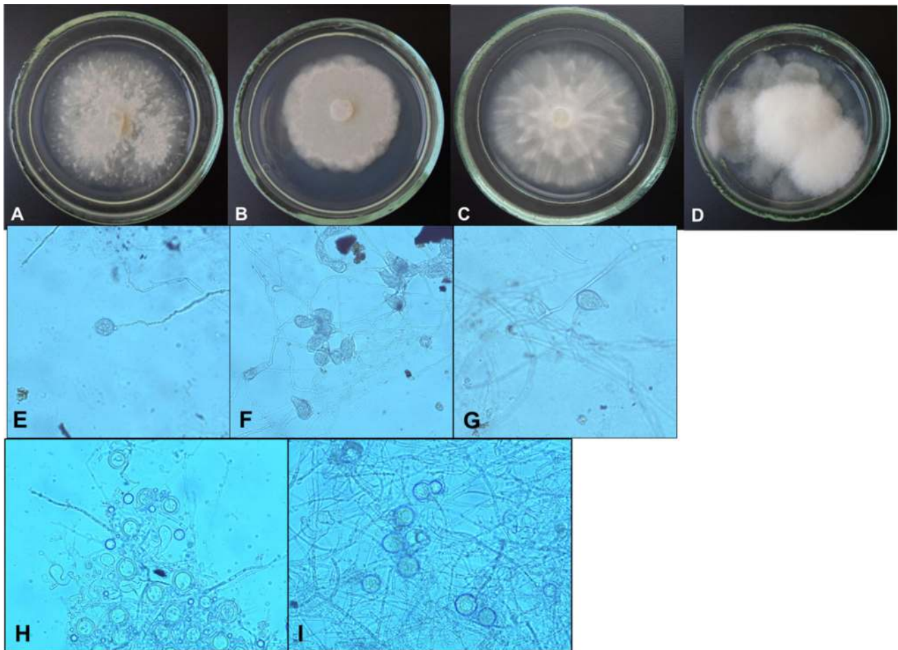
Fig. 1 Macroscopic and microscopic features of Phytophthora spp. growing in cultures on potato dextrose agar (PDA). The colonies were photographed on the sixth day of incubation: a P. citricola (isolate WG1), b P. cactorum (isolate BT1), c P. citrophthora (strain RH04/CTPH), and d P. cryptogea (isolate from Zarzecze). Morphology of
