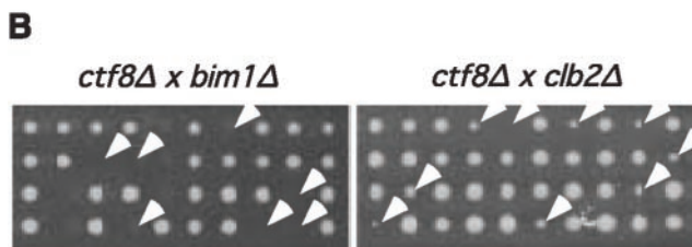
Figure 1. CTF8 genetic interactions. (A) Results from SGA analysis with ctf8Δ presented as a genetic interaction map. Lines represent a confirmed synthetic sick interaction between the connected genes. Broken lines represent synthetic lethal interactions. Gene functions are indicated. Genes required for efficient sister chromatid cohesion are indicated in bold. (B) Examples of tetrad analyses for a synthetic lethal interaction ( ctf8Δ bim1Δ ) and a synthetic sick interaction ( ctf8Δ clb2Δ ). Double mutants are indicated by the arrowheads.
