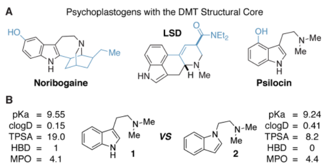
Figure 1. Structures of compounds possessing the DMT pharmacophore. (A) The DMT structure (highlighted in black) is the core scaffold of several known psychoplastogenic compounds. (B) The only difference between the chemical structures of DMT ( 1 ) and N,N -dimethylaminoisotryptamine (isoDMT) ( 2 ) is that the C1 and C3 substituents of the indole are transposed. Predicted chemical properties and calculated MPO scores are shown. clogD = calculated \log D ; TPSA = total polar surface area; HBD = hydrogen bond donor; and MPO = multiparameter optimization score.
