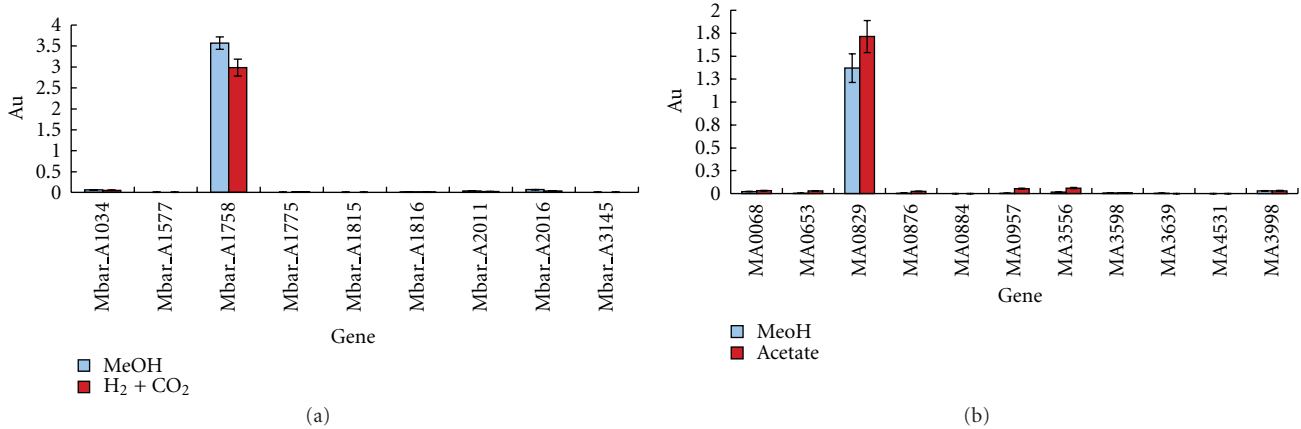
FIGURE 2: Expression of M. acetivorans and M. barkeri paralogous S-layer genes. (a) The Mbar_A1758-related genes in M. barkeri . (b) The MA0829-related genes in M. acetivorans . Abundance values (AU) are expressed in copy number [12]. Cells were grown with methanol (MeOH), acetate, or hydrogen and carbon dioxide (H 2 + CO 2 ) as the sole carbon and energy supply as described in Section 2.
