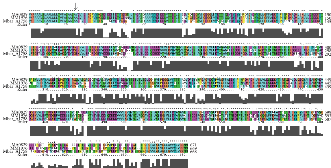
FIGURE 6: Primary amino acid alignment of the three major Methanosarcina S-layer proteins, Mbar_A1758, MA0829, and MM1976. Identity of the sequences is indicated by asterisks. The experimentally determined mature N-terminus for Mbar_A1758 (Section 3) is indicated by the arrow.
