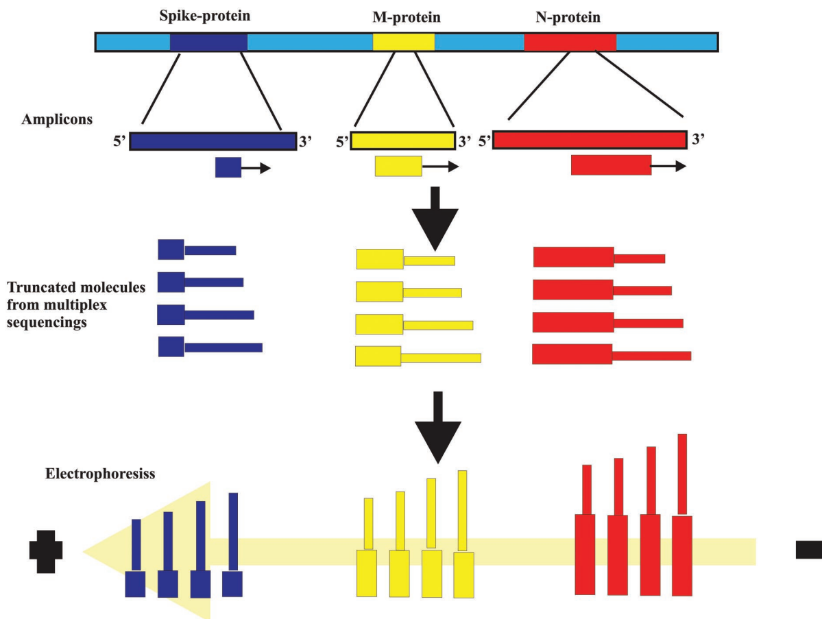
FIG. 1. Stages of the MultiGEN process and the basic scientific principles. These include simultaneous generation of three amplicons from the spike protein-encoding gene, gene M, and gene N and simultaneous sequencing of the 3' end of each of the amplicons.
