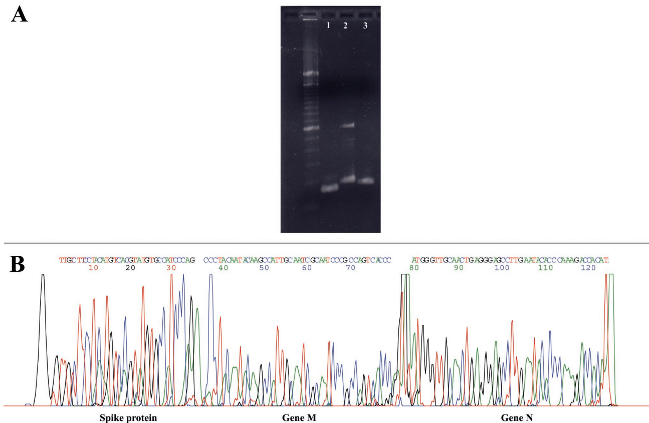
FIG. 2. (A) Agarose gel electrophoresis showing amplicons. Lane 1, spike gene amplicon (158 bp); lane 2, gene M amplicon (190 bp); lane 3, gene N amplicon (176 bp). (B) Electropherogram showing nucleotide sequences from three regions of the SARS-CoV genome: the spike protein-encoding gene (35 nucleotides), gene M (43 nucleotides), and gene N (45 nucleotides).
