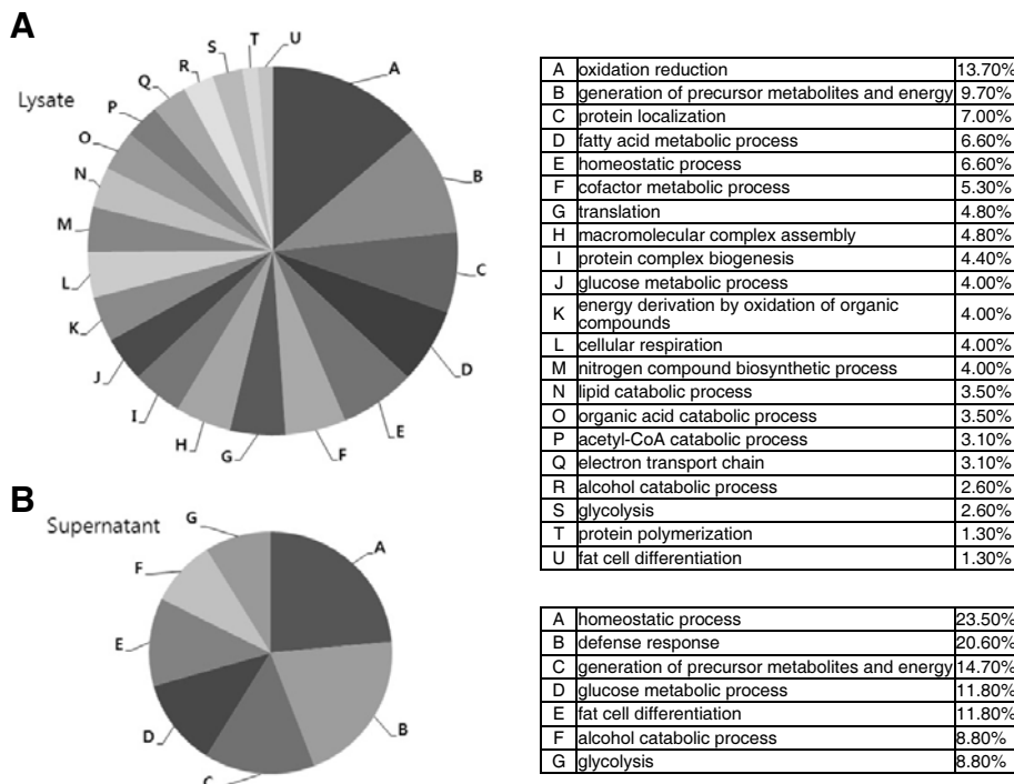
Fig. 3. Functional analysis of proteins differentially expressed from each proteome. The categories of proteins were generated using the program provided by the DAVID GO tool for (A) differential expressed proteins from the cytosolic fraction and (B) differential expressed proteins from secreted fraction.
