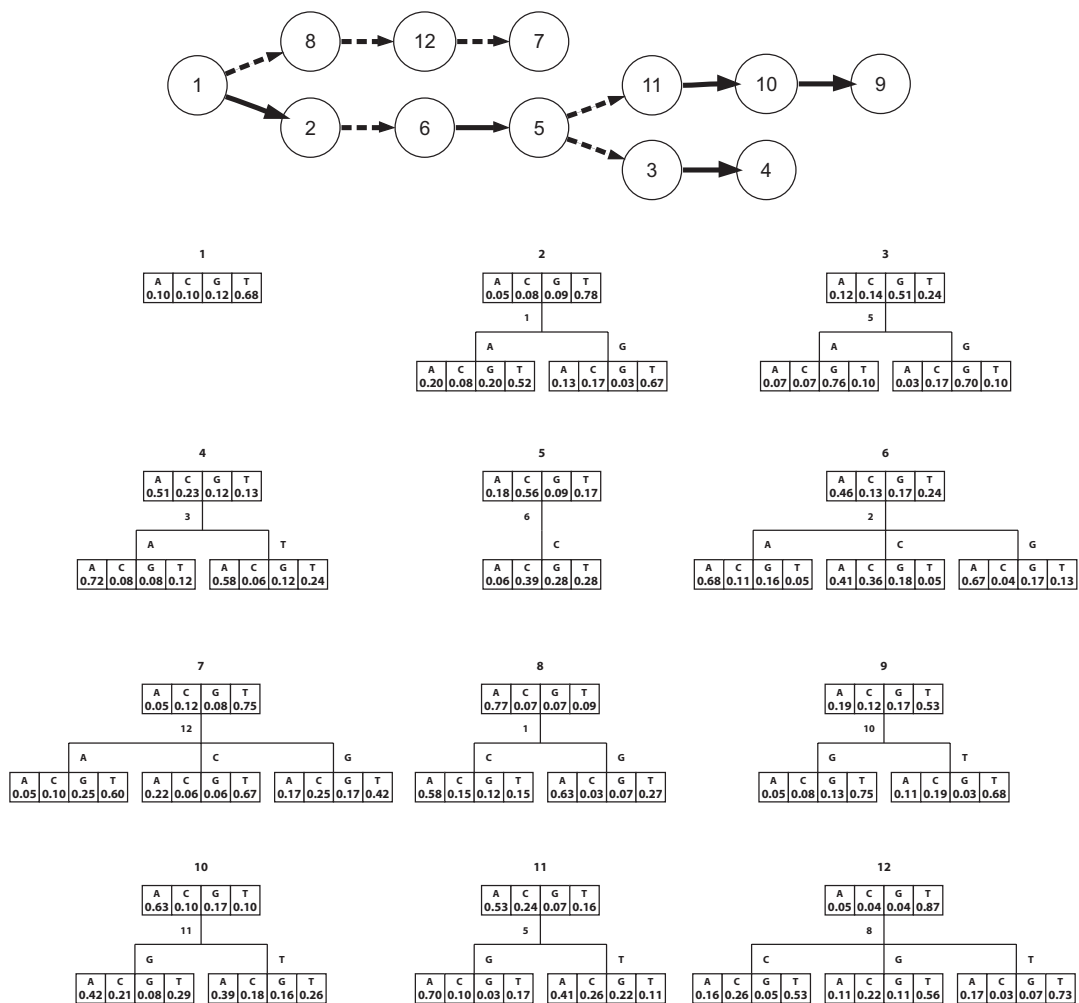
Fig. 3. The BT/BN(1) dependence graph and the corresponding VOBN(1, 2 -3.75 ) forest, as constructed from the sigma-70 foreground dataset. In the dependence graph (top) the solid lines represent adjacent positions and the dashed lines represent non-adjacent positions. In the VOBN forest, the nodes are labeled with the unconditional probability vector of nucleotides at that position in the box. The position is denoted by the upper numerical label (above the root). The position in the context of which we split is labeled by the numerical label near the split. Nodes 1–6 represents the ‘-35 box’ and nodes 7–12 represents the ‘-10 box’.
