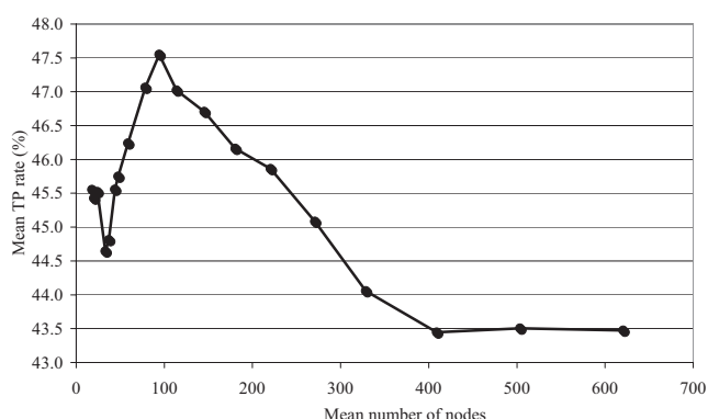
Fig. 6. Pruning the background VOM( 5, c ) model for different values of the pruning constant c . The foreground model is the VOBN( 1, 2^{-3.75} ) model, which was found to be the best model in Figure 5 and has \sim 36 nodes. The number of nodes in the background model is presented on the abscissa to show the size of the model.
