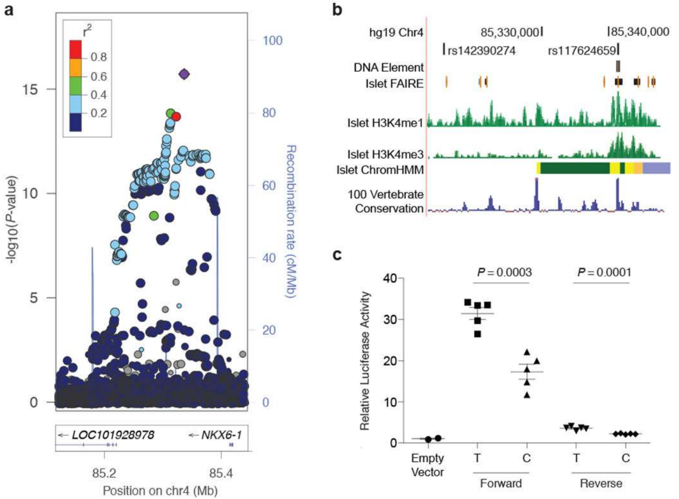
Figure 3: rs117624659 at NKX6-1 locus exhibits allelic differences in transcriptional activity. (A) rs117624659 ( N_{\text{eff}}=211,214 ; purple diamond) shows the strongest association with T2D in the region. P values were from two-sided fixed-effect inverse-variance meta-analysis. Variants are colored based on 1000G Phase 3 East Asian LD with rs117624659. (B) rs117624659 and an additional candidate variant rs142390274 in high pairwise LD ( r^2>0.80 ) span a 22 kb region approximately 75 kb upstream of NKX6-1 . rs117624659 overlaps a region of open chromatin in pancreatic islets and lies within a region conserved across vertebrates. (C) rs117624659-T, associated with increased risk of T2D, showed greater transcriptional activity in an element cloned in both forward and reverse orientations with respect to NKX6-1 in MIN6 cells compared to rs117624659-C and an “empty vector” containing a minimal promoter. Black lines represent mean (center horizontal line) and standard error (extended lines) relative luciferase activity from two-sided, unpaired t-tests using data from n=5 biologically independent samples/independent experiments.
