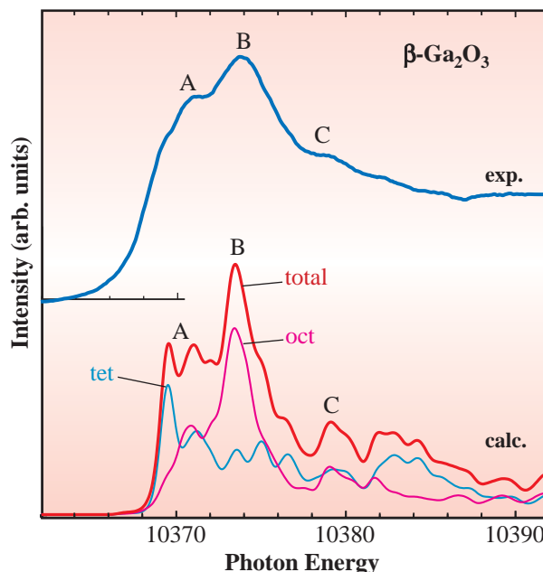
Fig. 1. Comparison of experimental and theoretical Ga-K-edge NEXAFS of \beta -Ga 2 O 3 . Theoretical spectra denoted by tet and oct correspond to spectra for Ga atoms at tetrahedral and octahedral sites, respectively. The sum of the two spectra is shown as total.
