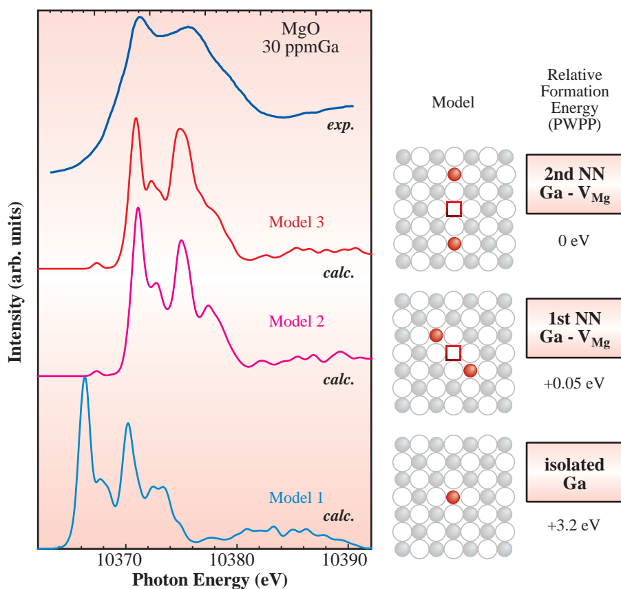
Fig. 2. Comparison of experimental and theoretical Ga-K-edge NEXAFS of Ga in MgO. Theoretical formation energies per Ga atom in MgO obtained by the PWPP calculations for the three models are shown together.
