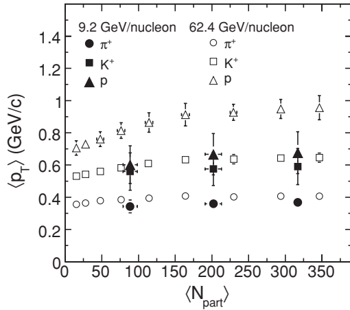
FIG. 12. \langle p_T \rangle for \pi^+ , K^+ , and p plotted as a function of \langle N_{part} \rangle for Au + Au collisions at \sqrt{s_{NN}} = 9.2 GeV and compared with corresponding results at \sqrt{s_{NN}} = 62.4 GeV [4,23,37]. The errors shown are the quadrature sum of statistical and systematic uncertainties. The systematic errors for pions, kaons, and protons for \sqrt{s_{NN}} = 9.2 GeV are \sim 12\% , 18\% , and 21\% , respectively, and similar for all the collision centralities studied.
