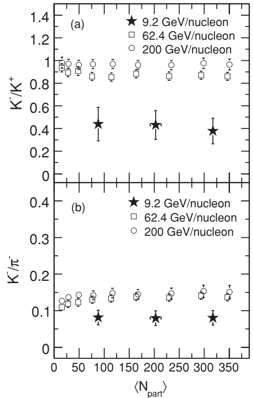
FIG. 14. Variation of (a) K^-/K^+ and (b) K^-/\pi^- ratios as a function of \langle N_{part} \rangle for Au + Au collisions at \sqrt{s_{NN}} = 9.2 GeV. For comparison we also show the corresponding results from Au + Au collisions at \sqrt{s_{NN}} = 62.4 and 200 GeV [23,37]. The errors shown are the quadrature sum of statistical and systematic uncertainties. The systematic errors for K^-/K^+ and K^-/\pi^- for \sqrt{s_{NN}} = 9.2 GeV data are \sim 25\% and 22\% , respectively, and similar for all the collision centralities studied.
