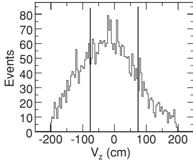
FIG. 1. Event-by-event distribution of the z position of the primary vertex V_z in Au + Au collisions at \sqrt{s_{NN}} = 9.2 GeV. The vertical solid lines show the condition of |V_z| < 75 cm for selected events.
