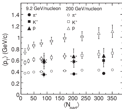
FIG. 13. \langle p_T \rangle for \pi^+ , K^+ and p plotted as a function of \langle N_{part} \rangle for Au + Au collisions at \sqrt{s_{NN}} = 9.2 GeV and compared with corresponding results at \sqrt{s_{NN}} = 200 GeV [4,23,37]. The errors shown are the quadrature sum of statistical and systematic uncertainties. The systematic errors for pions, kaons, and protons for \sqrt{s_{NN}} = 9.2 GeV are \sim 12\% , 18\% , and 21\% , respectively, and similar for all the collision centralities studied.
