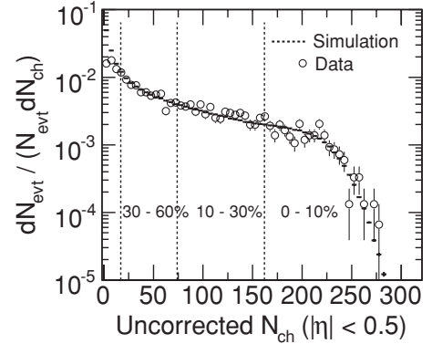
FIG. 3. Uncorrected charged-particle multiplicity distribution (open circles) measured in the TPC within |\eta| < 0.5 in Au + Au collisions at \sqrt{s_{NN}} = 9.2 GeV. The dashed histogram represents the simulated multiplicity distribution. The vertical dashed lines reflect the centrality selection criteria used in the paper. Errors are statistical only.
