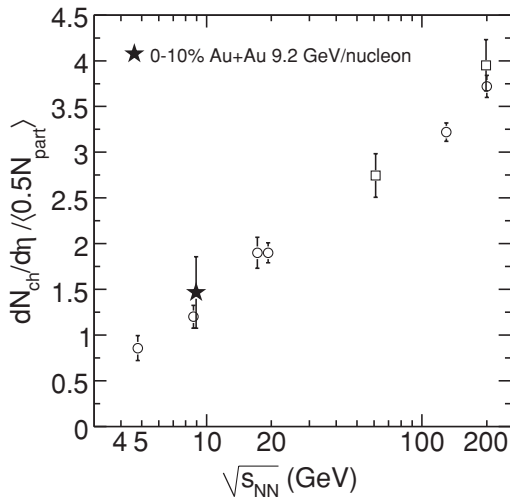
FIG. 16. Midrapidity dN_{\text{ch}}/d\eta normalized by \langle N_{\text{part}} \rangle/2 as a function of \sqrt{s_{NN}} . Au + Au collisions at \sqrt{s_{NN}} = 9.2 GeV are compared with previous results from AGS [38], SPS [39], and RHIC [23,40]. The errors shown are the quadrature sum of statistical and systematic uncertainties. The systematic error for \sqrt{s_{NN}} = 9.2 GeV data is 39\% .
