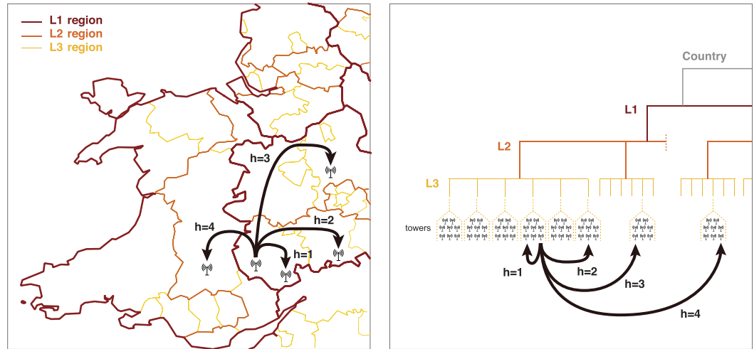
Figure 1. Partitioning of a country based on telephone call networks. Hierarchical distances between two locations are defined through three regional levels - either administrative ones or those found by applying iterative community detection on human interaction networks. Two distinct locations are at a hierarchical distance h = 1 , if they are in the same L_3 region, h = 2 , if they are in different L_3 regions but in the same L_2 region, h = 3 , if they are in different L_2 regions but in the same L_1 region and h = 4 , if they are in different L_1 regions. Note that a higher hierarchical distance does not necessarily correspond to higher geographical distance. The figure has been created using Matlab R2015b ( http://www.mathworks.com ) and publicly available shapefile data for the regional borders ( http://ec.europa.eu/eurostat/web/gisco/geodata/reference-data/administrative-units-statistical-units , (c) EuroGeographics, 2016).
