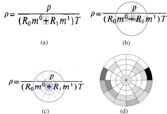
Fig. 3. Example: Calculating layout context for "+," using r = 4 and 5 key points (bounding box corners and center). (a) Expression where the reference symbol "+" lies. (b) Vectors that connect other key points within the neighborhood to the bounding box center. (c) 60 log polar bins of the circle neighborhood area. (d) Visual representation of the layout context of symbol "+". Darker bins contain more points.
