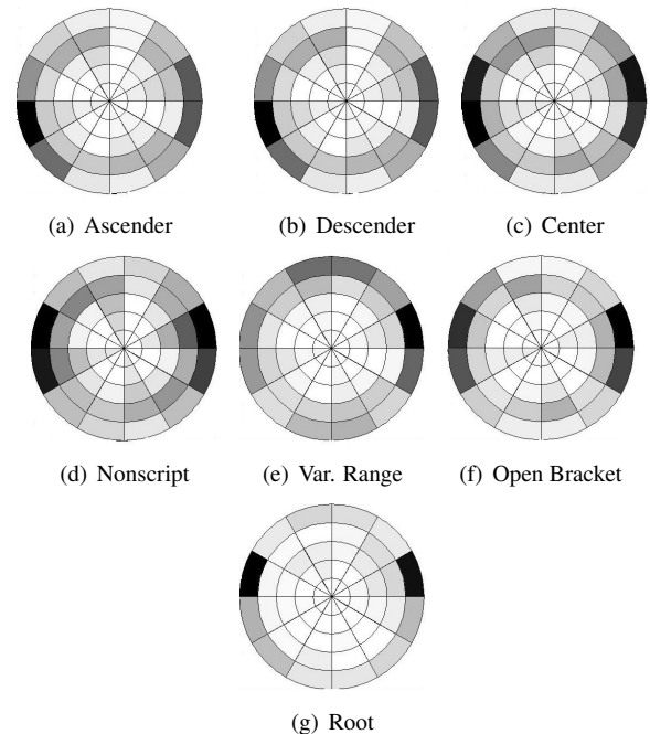
Fig. 4. Average layout context histogram for each layout class
