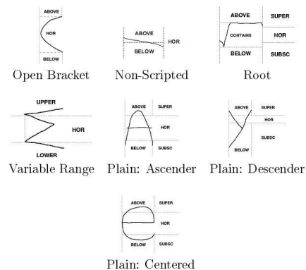
Fig. 1. Symbol layout classes [5]
