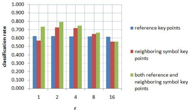
Fig. 6. Comparison of highest classification rates for key points taken from the reference symbol alone, neighborhood symbols alone, and both reference and neighbor symbols for different neighborhood sizes ( r )
