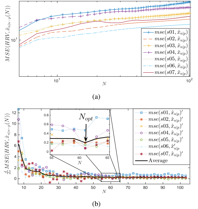
Figure 1: Estimation of optimal horizon as N_{\text{opt}} = 61 : a) MSE of HRV/seizures data (s01, s02,..., s07) for the estimate x_{n|n-p}(N) and b) minimization of \partial\eta(N)/\partial N to solve the optimization problem (4).
