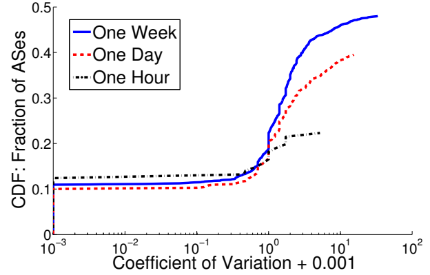
Figure 4: CV of Pkt Loss Rate for ASes
