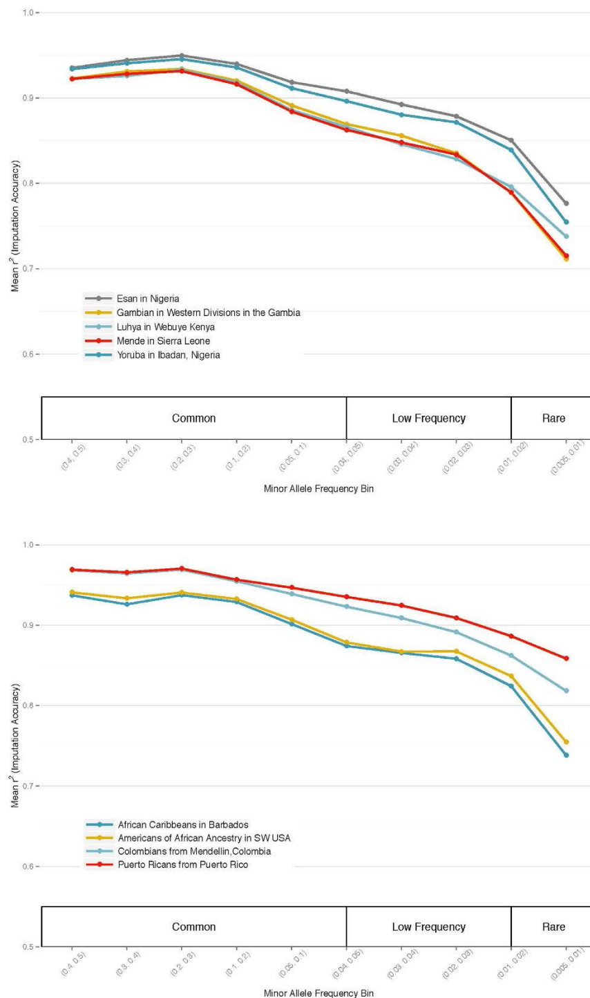
Figure 2. Estimated imputation coverage of variants tagged by the ADPC content as part of the MEGA array. (a) Coverage in 1000 Genomes African populations is \geq 0.8 r^2 down to 1% MAF. (b) Coverage in 1000 Genomes admixed African populations is \geq 0.8 r^2 down to 1% MAF
