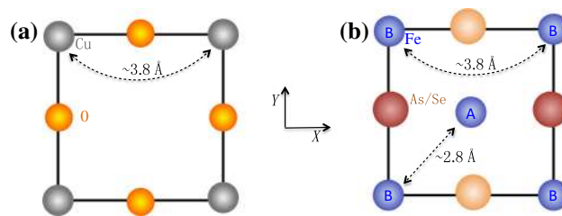
Fig. 1 (Color online) The comparison of the lattice unit cells between cuprates and iron-based superconductors. a The unit cell and lattice constant of the \text{CuO}_2 layer in cuprates; b The unit cell and lattice constant of the FeAs/Se layer which includes two irons marked as A and B
