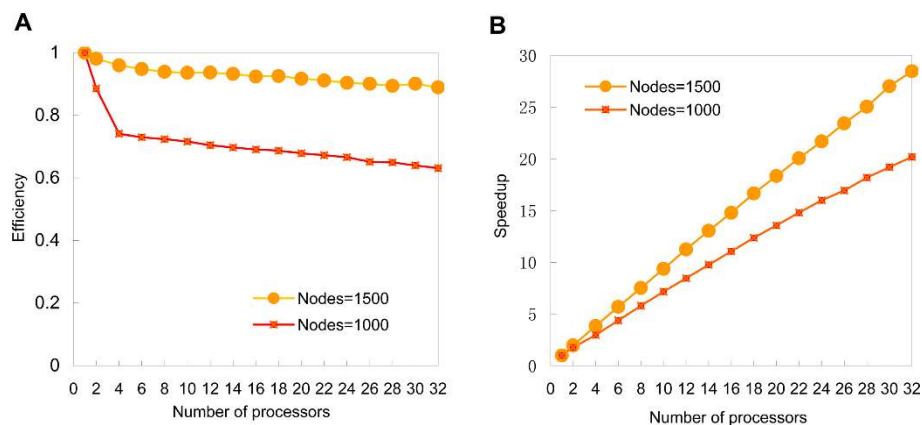
Figure 1 The efficiency and speedup curves of the parallel SWNI algorithm. Both of the efficiency and speedup are calculated on two samples. One is an network of 1000 nodes and the other is an network of 1500. (A) Efficiency of the algorithm draw dramatically when processors increased from one to four and then tend to stable. (B) The Speedup is close to a straight line with network of 1500 nodes compared to the network of 1000 nodes.
