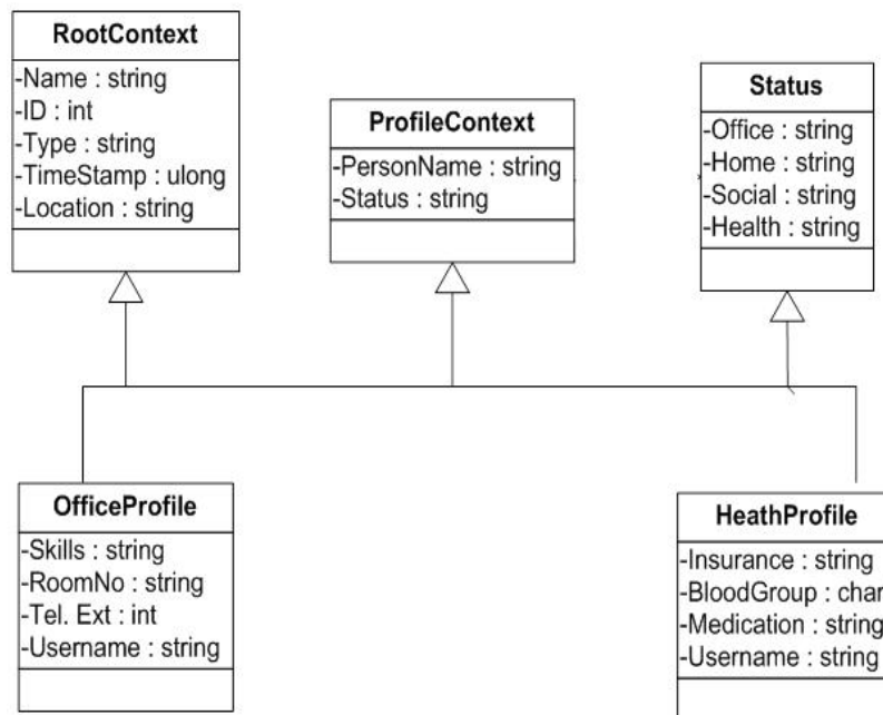
Figure 4. XML Schema
