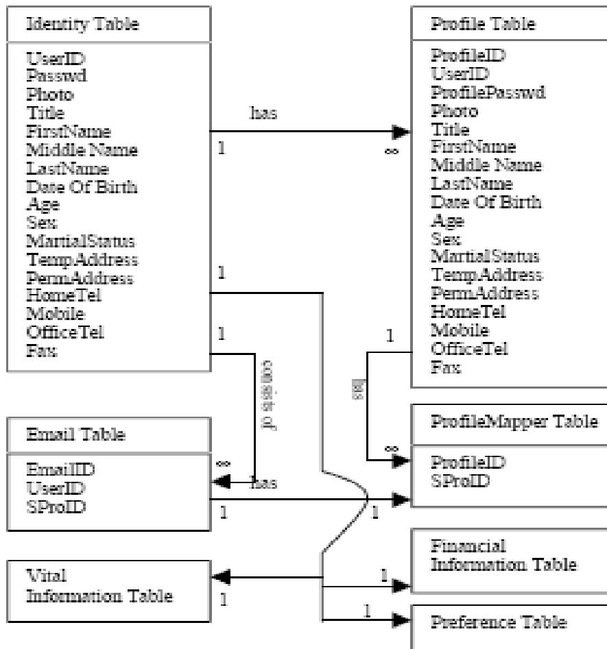
Figure 3. Identity Attributes
