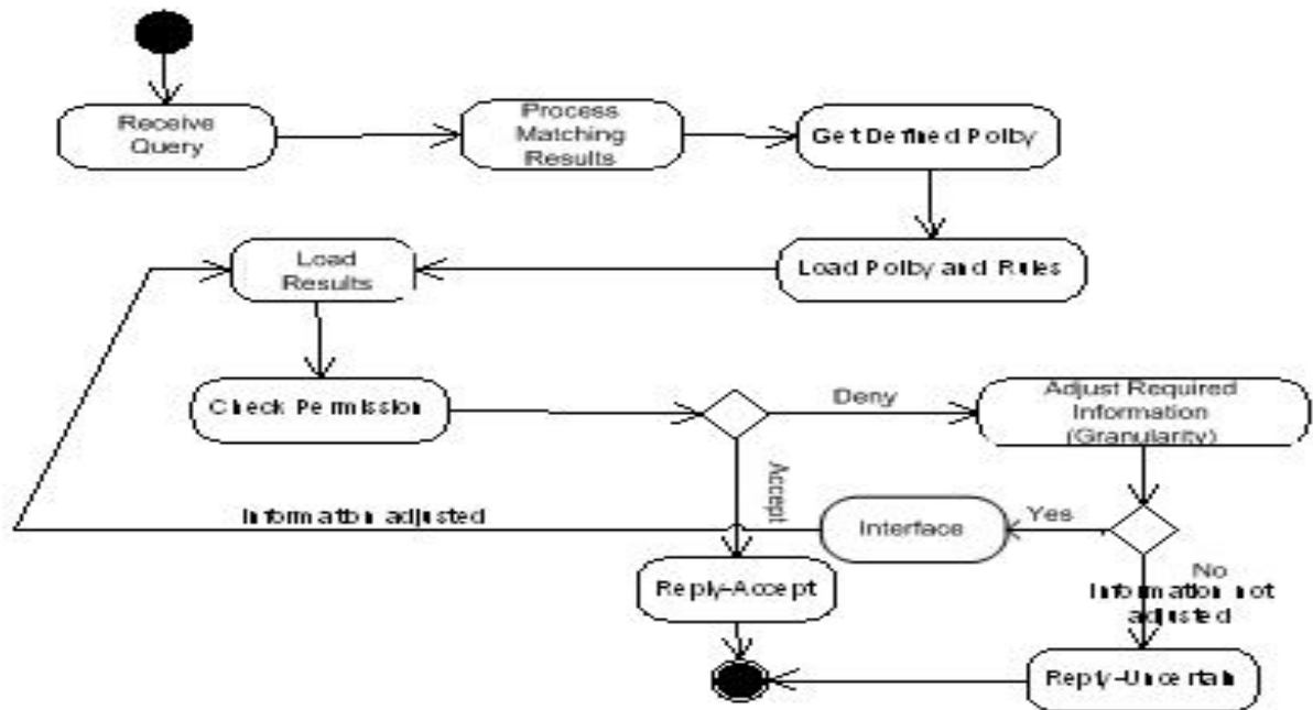
Figure 2. Information Granularity
