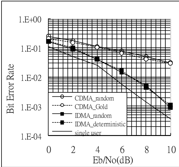
Figure 4. BER of four-user IDMA and CDMA systems in three-path Rayleigh fading channels, iteration=3.
