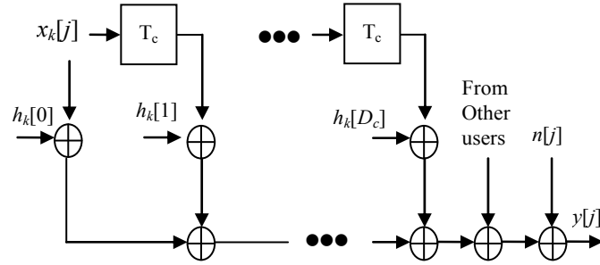
Figure 2. The multipath channel model, where D_c is the number of paths.
