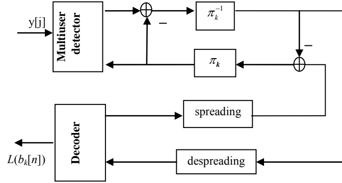
Figure 3. The receiver model for user k . The multiuser detector and channel decoder exchange extrinsic information using the turbo principle.
