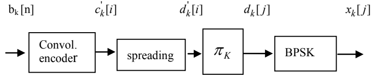
Figure 1. The transmitter model for user k .
