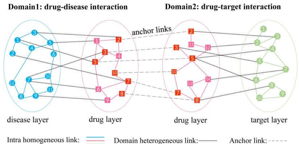
Fig 1. An overview of iDrug. An illustration of the cross-network framework across two domains: drug-disease and drug-target networks. iDrug requires only partially overlapped drug nodes between these two domains. The anchor links among drug nodes are used to transfer domain knowledge across the networks.
