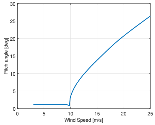
(b) Pitch angle
