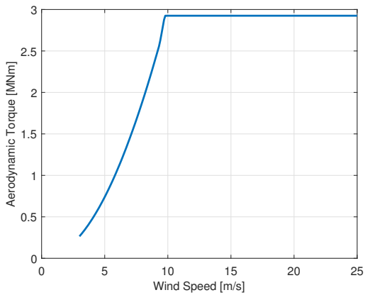
(e) Aerodynamic torque
