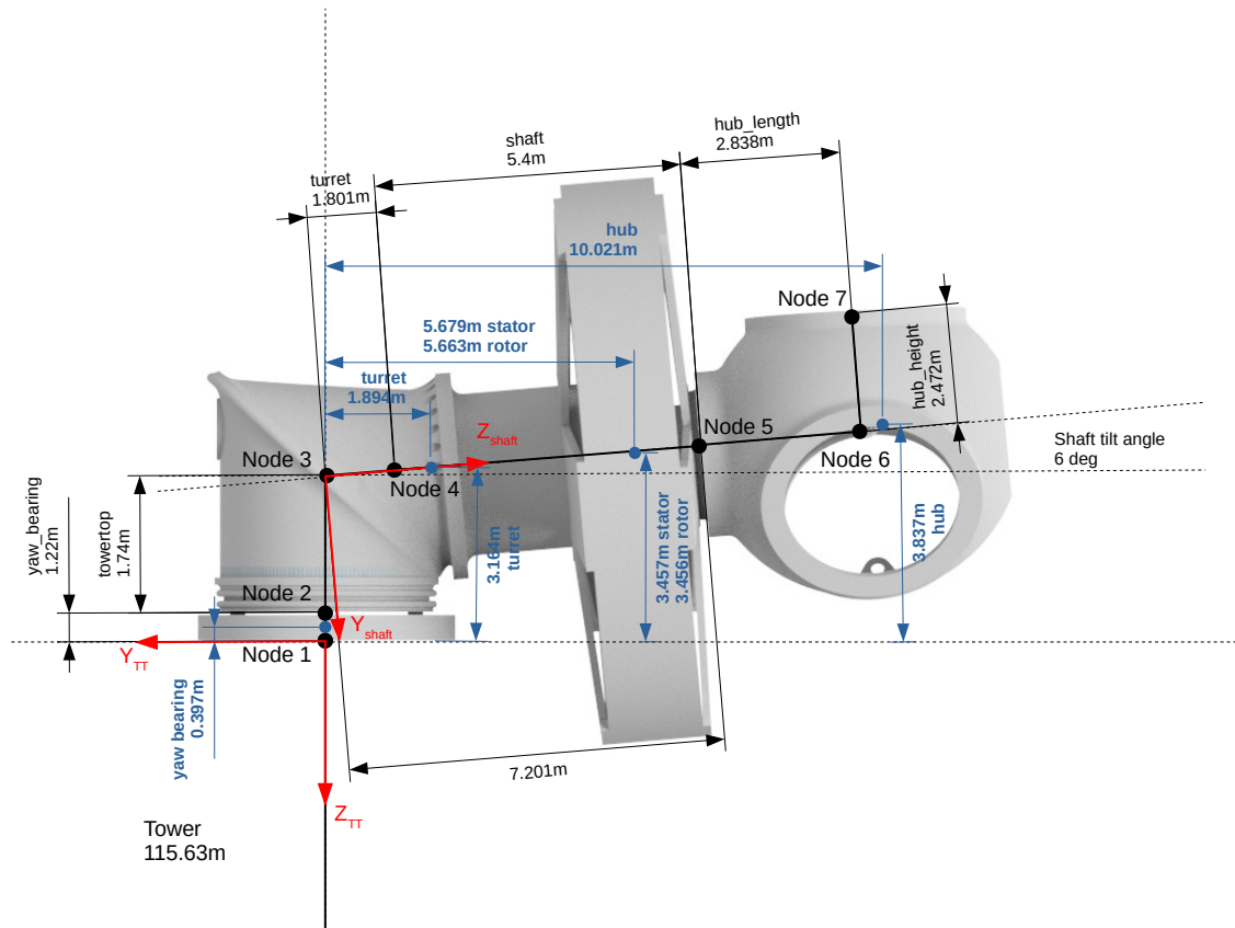
Figure 37: Beam model representation of the nacelle assembly. The location of the lumped masses are given in blue.
