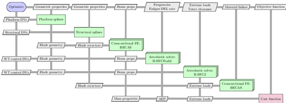
Figure 5: Extended design structure matrix diagram of the workflow of HAWTOpt2.
