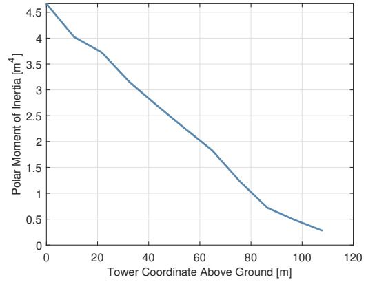
(b) Polar moment of inertia distribution
