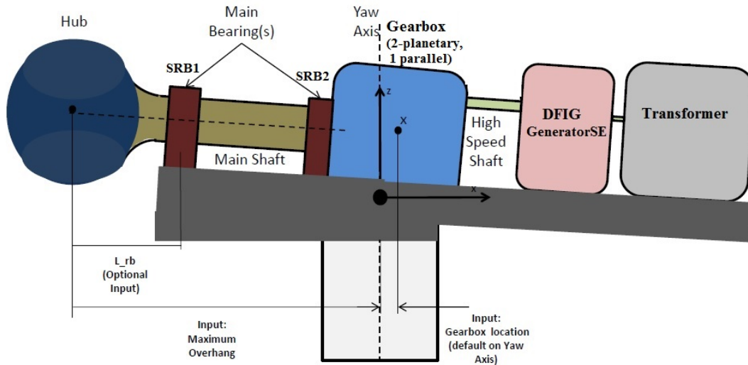
Figure 13: Drivetrain layout.
