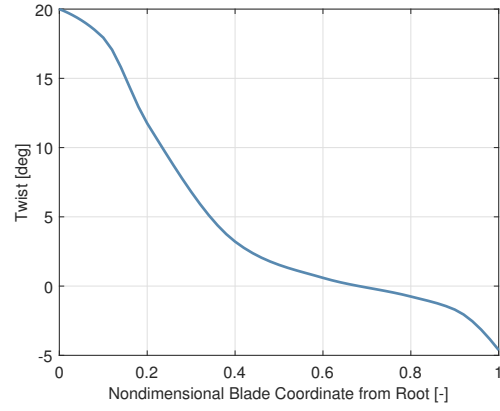
(b) Twist
