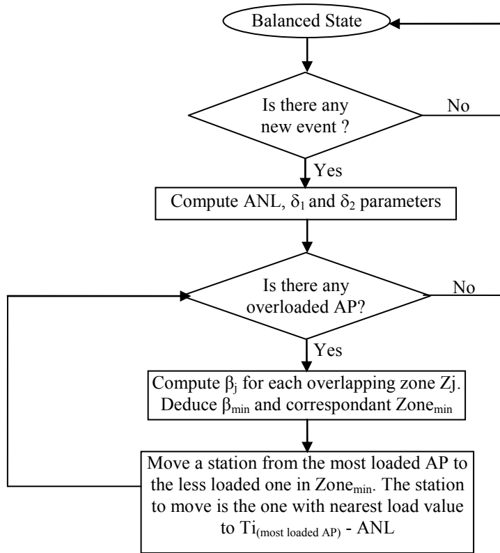
Figure 3 General diagram of the Load Balancing Algorithm
