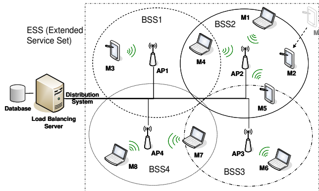
Fig. 1. IEEE 802.11 target architecture
