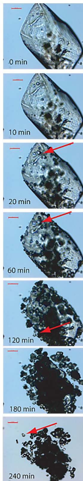
Fig. 5. Ikaite crystal dissolution during melting of sea ice over 240 min. Arrows point at smaller sub-units of crystals (also ikaite) that emerge during melting. Scale bar is 50 μm.
