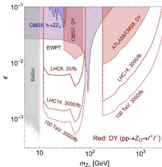
Figure 8. Prospects for Z_D searches from DY production (red lines) at LHC8 ( 20\text{ fb}^{-1} , solid), LHC14 ( 3000\text{ fb}^{-1} , dashed), and a 100 TeV pp collider ( 3000\text{ fb}^{-1} , dotted), with limits from existing recasts shown in shaded red (from [71, 72, 136, 137] and our rescalings, see text for details). A recast [67] of a CMS8 analysis [122] sensitive to h \rightarrow ZZ_D is shown in the blue shaded region. The purple region shows the current EWPT constraints (this work, see Section 3), while the gray region is a limit from BaBar [61].
