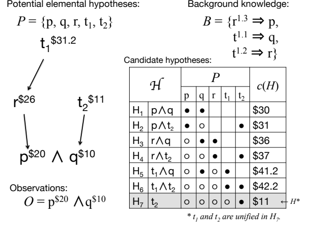
Figure 1: The combinatorial representation of candidate hypotheses by set P of potential elemental hypotheses. The black circle indicate that a proposition is in H_i , while the white circle indicate that a proposition is explained by H_i \cup B .
