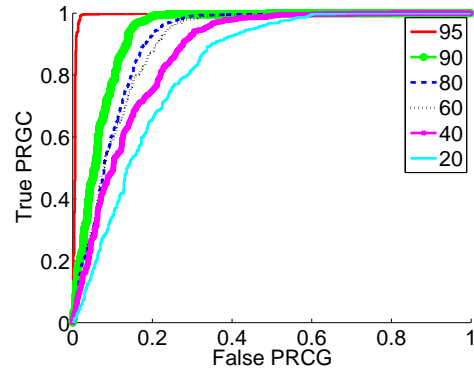
Figure 7. Our algorithm’s classification accuracy gracefully fades as a function of compression amount. Each curve reports the classification performance for distinguishing between PRGC and PIM on the ADVENT dataset for size different compression levels.
