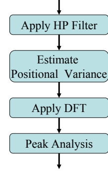
Figure 3. Flow diagram for detecting demosaicing. First a high-pass filter is applied, then the variance of each diagonal is estimated. Fourier analysis is used to find periodicities in the variance signal, indicating the presence of demosaicing.
