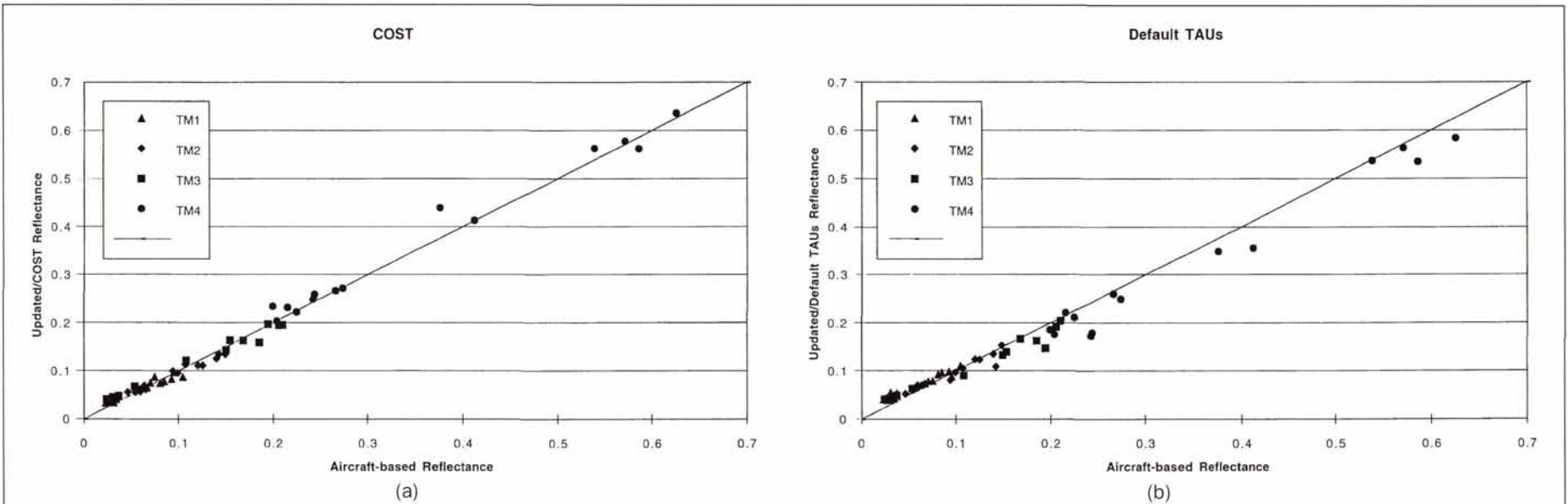
Figure 2. Results generated by the COST (a) and default TAU's (b) models on computed satellite-based versus measured aircraft-based reflectances for TM bands 1, 2, 3, and 4 using the soils and vegetation data for seven dates from 23 July 1985 to 24 June 1986 (Table 1).
