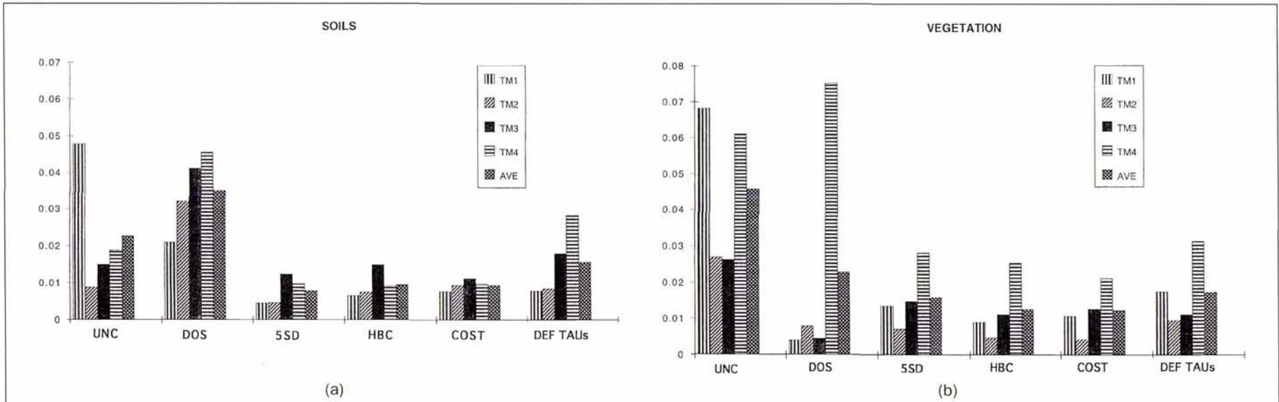
Figure 3. Reflectance results for spectral-bands TM 1, 2, 3, and 4 and an overall average, as determined by six models for the soils (a) and vegetation (b) targets. The average of the absolute difference between the computed and aircraft-based measured values are plotted.
