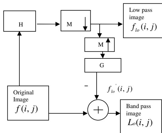
Figure 2: One level LP decomposition
