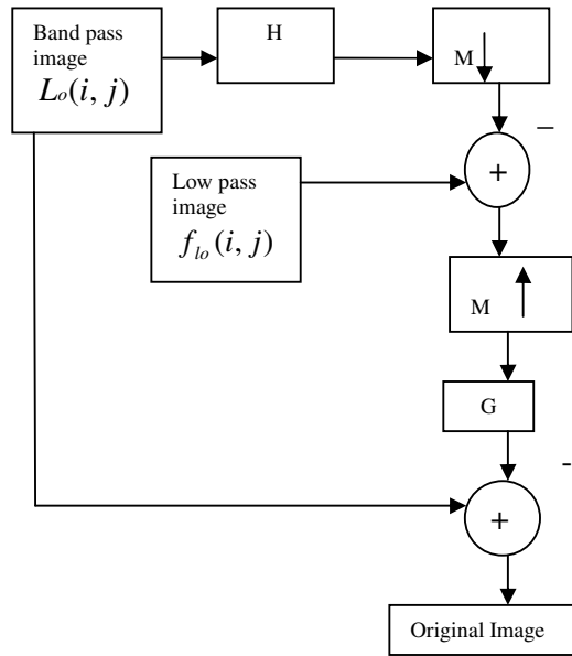
Figure 3: One level LP reconstruction
