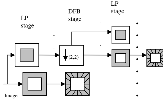
Figure 1: Contourlet Filter bank
