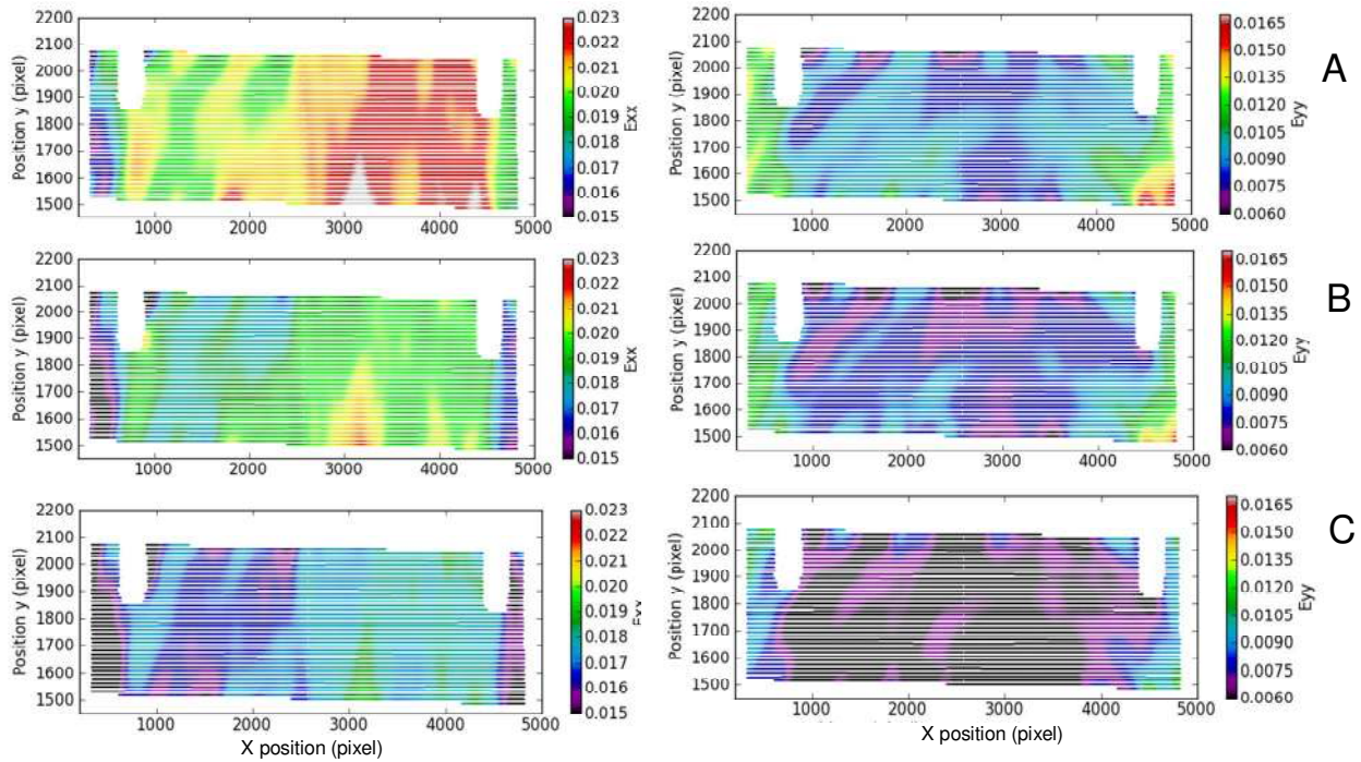
Hygrothermal loading Strain evolution of poplar flatsawn sample at 90% RH (A) At T1 (cf. Figure 3) (B) At T4 (C) At T7
