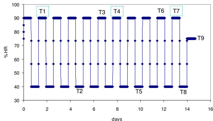
Figure 3 – Relative humidity cycles
