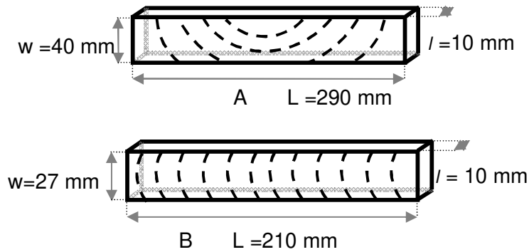
Figure 2 – Specimen sizes. (A) flatsawn. (B) Quartersawn
