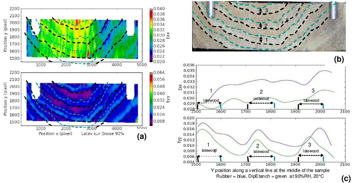
Figure 6 – Strain distribution on a flatsawn sample at 90%RH
