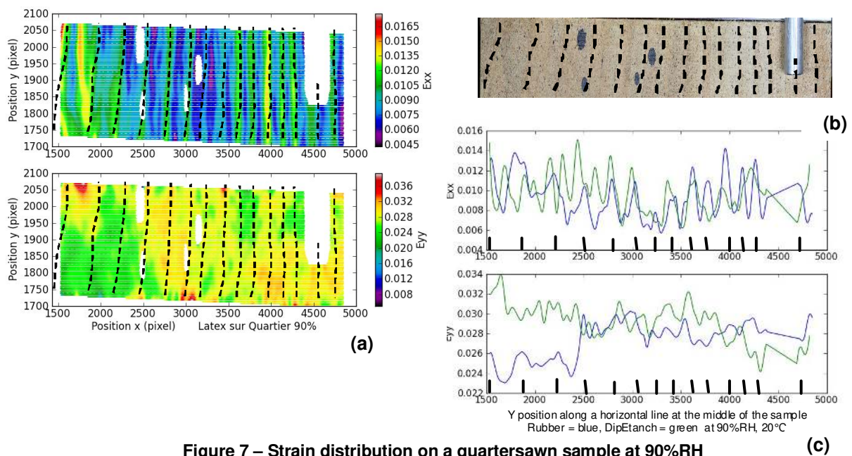
Figure 7 – Strain distribution on a quartersawn sample at 90%RH
