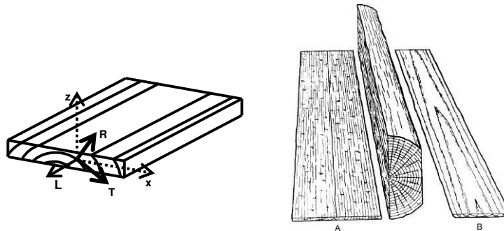
Figure 1 – Wood panel, orthotropic orientation Quartersawn (A) and flatsawn (B) boards cut from a log
