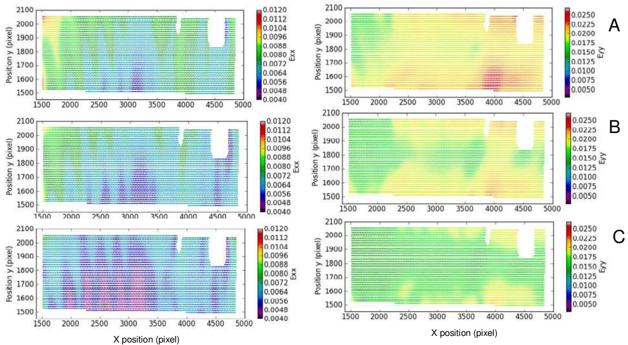
Hygrothermal loading Strain evolution of quartersawn poplar sample at 90% RH (A) At T1 (cf. Figure 4) (B) At T4 (C) At T7
