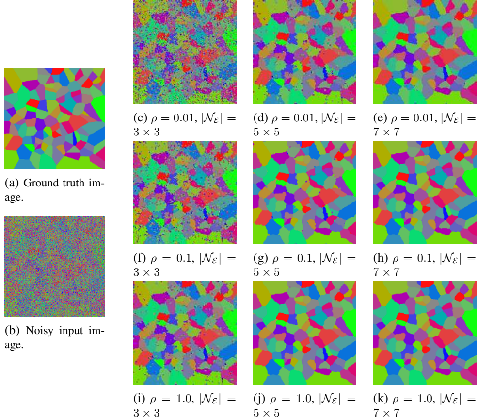
FIGURE 4.2. Parameter influence on labeling. Panels (a) and (b) show a ground-truth image and noisy input data. Both images and the prior data set \mathcal{P}_\mathcal{F} are composed of 31 color vectors. Each color vector is encoded as a vertex of the simplex \Delta_{30} . This results in unit distances between all colors and thus enables an unbiased assessment of the impact of geometric averaging and the two parameter values \rho, |\mathcal{N}_\varepsilon| . Panels (c)-(k) show the assignments u(W^*) for various parameter values where W^* maximizes the objective function (3.16). The spatial scale |\mathcal{N}_\varepsilon| increases from left to right. The results illustrate the compromise between sensitivity to noise and to the geometry of signal transitions. The selectivity parameter \rho increases from top to bottom. If \rho is chosen too small, then there is a tendency to noise-induced oversegmentation, in particular at small spatial scales |\mathcal{N}_\varepsilon| . Note, however, that depending on the application, the ability to separate the physical and the spatial scale in order to recognize outliers with small spatial support, while performing diffusion at a larger spatial scale as in panels (c),(d),(f),(i), may be beneficial. We point out that this separation of the physical and spatial scales (image range vs. image domain) is not possible with total variation based regularization where these scales are coupled through the co-area formula. All results were computed using the assignment mapping (3.20) without rounding. This shows that the termination criterion of Section 3.3.4, illustrated by Figure 4.1 leads to (almost) unique assignments.
