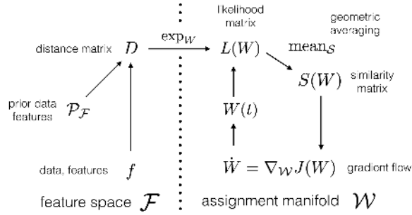
FIGURE 1.1. Overview of the variational approach. Given data and prior features in a metric space \mathcal{F} , inference corresponds to a Riemannian gradient flow with respect to an objective function J(W) on the assignment manifold \mathcal{W} . The curve of matrices W(t) assigns at each t prior data \mathcal{P}_{\mathcal{F}} to observed data f and terminates at a global maximum W^* that constitutes a labeling, i.e. a unique assignment of a single prior datum to each data point. Spatial coherence of the labeling field is enforced by geometric averaging over spatial neighborhoods. The entire dynamic process on the assignment manifold achieves a MAP-labeling in a smooth, geometrical setting, realized with sparse interior-point numerics in terms of parallel multiplicative updates.
