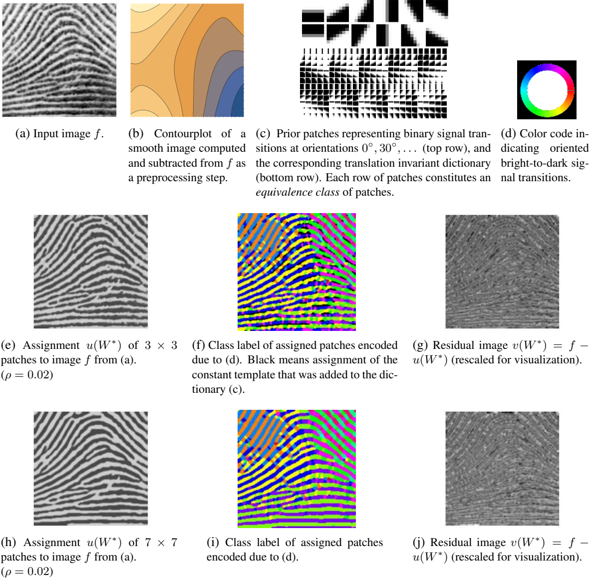
FIGURE 4.5. Analysis of the local signal structure of image (a) by patch assignment. This process is twofold non-local: (i) through the assignment of 3 \times 3 patches (center row) and 7 \times 7 patches, respectively, and (ii) due to the gradient flow (3.21) that promotes the spatially coherent assignment of patches corresponding to different orientations of signal transitions, in order to maximize the similarity objective (3.16).
