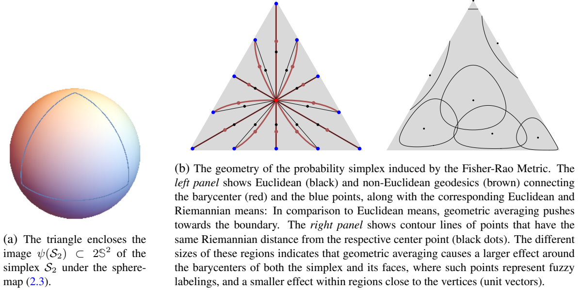
FIGURE 2.1. Geometry of the probability simplex \mathcal{S}_2 .
