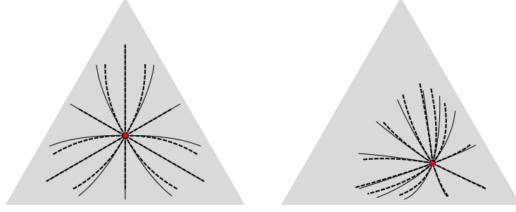
FIGURE 3.1. Illustration of Prop. 3.1. Various geodesics \gamma_{v^i}(t) , i \in [k] , t \in [t, t_{\max}] (solid lines) emanating from p (red point) with the same speed \|v^i\|_p = \|v^j\|_p , \forall i, j , are displayed together with the curves \exp_p(u^i t) , i \in [k] , t \in [t, t_{\max}] , where the vectors u^i, v^i , i \in [k] satisfy (3.9).
