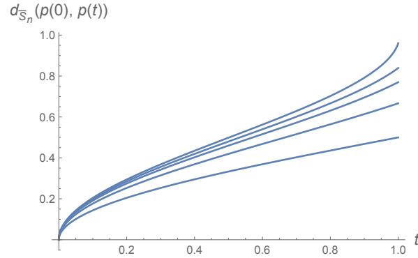
FIGURE 2.2. Each curve represents the Riemannian distances d_{\bar{\mathcal{S}}_n}(p(0), p(t)) (normalized to [0,1] ; Eq. (2.4)) of points on the curve \{p(t)\}_{t \in [0,1]} that linearly (i.e., Euclidean) interpolates between the fixed vertex p(0) = e^1 of the simplex \bar{\mathcal{S}}_n = \Delta_{n-1} and the barycenter p(1) = \bar{p} , for dimensions n = 2^k , k \in \{1, 2, 3, 4, 8\} . As the dimension n grows, the barycenter is located as far away from e^1 as all other boundary points e^i, te^i + (1-t)e^j , t \in [0, 1] , i, j \neq 1 , etc., which have disjoint supports. This entails a normalizing effect on the Riemannian mean of points that are far away, unlike with Euclidean averaging where this influence increases with the Euclidean distance.
