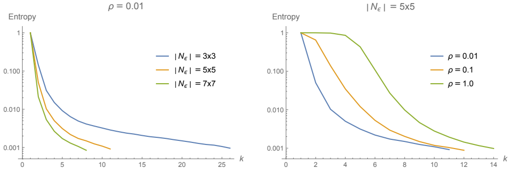
FIGURE 4.1. Parameter values and convergence rate. Average entropy (3.37) of the assignment vectors W_i^{(k)} as a function of the iteration counter k and the two parameters \rho and |\mathcal{N}_\epsilon| , for the labeling task illustrated by Figure 4.2. The left panel shows that despite high selectivity in terms of a small value of \rho , small spatial scales necessitate to resolve more conflicting assignments through propagating information by geometric spatial averaging. As a consequence, more iterations are needed to achieve convergence and a labeling. The right panel, on the other hand, shows that at a fixed spatial scale |\mathcal{N}_\epsilon| higher selectivity leads to faster convergence, because outliers are simply removed from the averaging process, whereas low selectivity leads to an assignment (labeling) taking all data into account.
