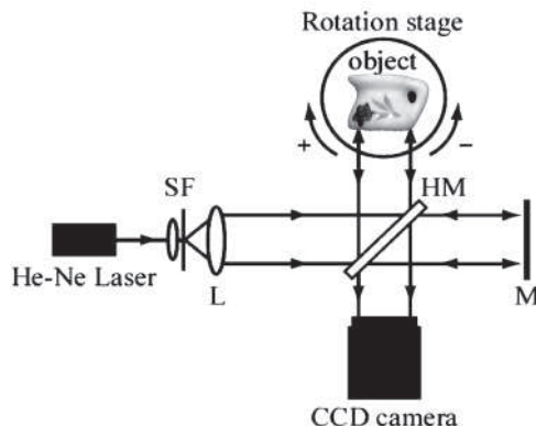
Fig. 11. An optical setup for digital hologram recording. SF: spatial filter, HM: half mirror, M: mirror, L: lens.
