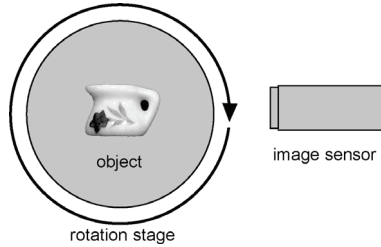
Fig. 8. Recording digital holograms by an image sensor on the concyclic positions.
