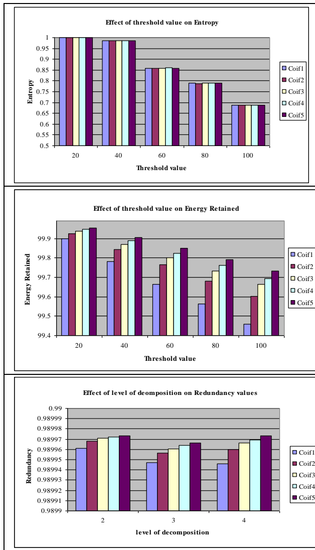
Figure 6: Experimental results of Coiflet wavelet family
