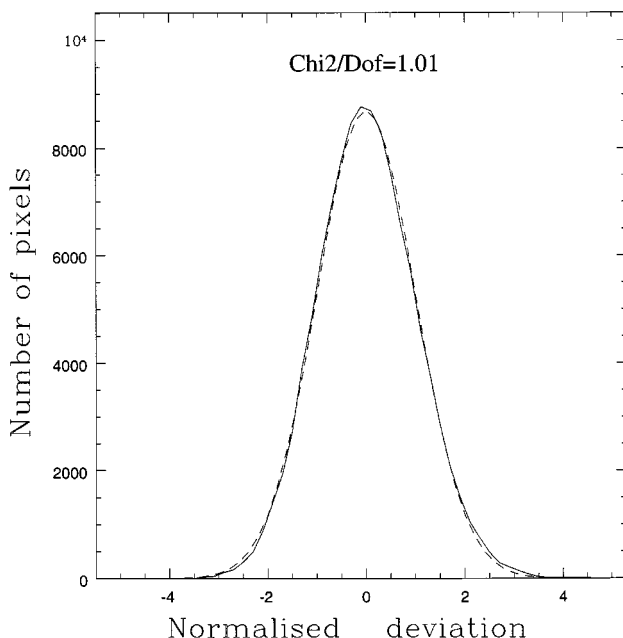
Fig. 6. Histograms of the deviations in the subtracted image in the case of very undersampled PSF's. The PSF in the reference image is very narrow with: FWHM = 1.17 pixels, thus we are in presence of a bad case of under-sampling. For the other image FWHM = 1.67 , consequently it is also under-sampled
