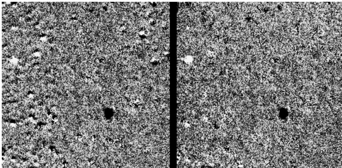
Fig. 7. Left is the subtracted image obtained with constant kernel solution. Note the systematic residuals around the bright objects on the left side of the image and in the upper right corner. Note the disappearance of these patterns in the next image, which has been obtained by fitting the spatial variations of the kernel to order 2. Two variables are present in the field (the bright and dark spots), and circular areas around these objects had to be excluded for \chi^2 evaluation
