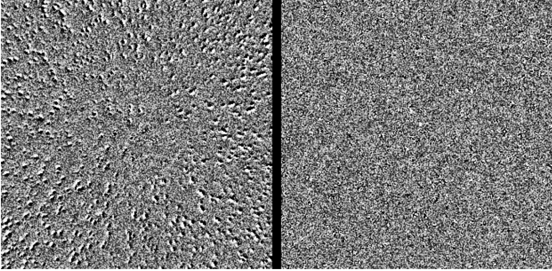
Fig. 4. Left is the subtracted image obtained with constant kernel solution. Note the systematic pattern due to the differential rotation between the images. Next is the subtracted image obtained by fitting the spatial variations of the kernel to order 2. Note the complete disappearance of the systematic patterns
