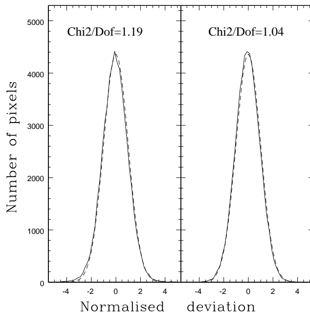
Fig. 8. Histograms of the normalized deviations in the subtracted images presented in Fig. 7. Left is the histogram for constant kernel solution, and right is the histogram for a fit of kernel variation to order 2. The dashed curve is Gaussian with \sigma = 1
