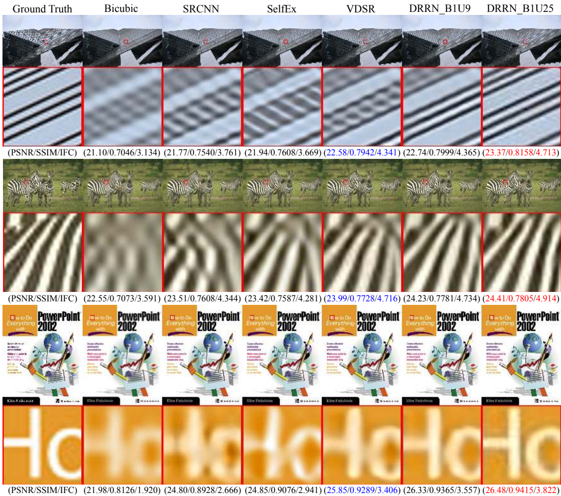
Figure 7. Qualitative comparison. (1) The first row shows image “img059” (Urban100 with scale factor \times 3 ). DRRN recovers sharp lines, while others all give blurry results. (2) The second row shows image “253027” (BSD100 with scale factor \times 3 ). DRRN accurately recovers the pattern. (3) The last row shows image “ppt3” (Set14 with scale factor \times 4 ). Texts in DRRN are sharp, while others are blurry.
