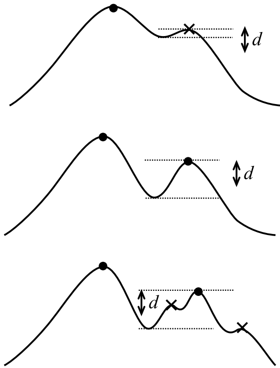
Figure 3. Schematic illustration of the criterion to depict the summits (highest points) of well-separated peaks. Plot is made for one-dimensional cases for simplicity. Filled circles represent the summits, and cross marks represent local bumps (non-summit local peaks), according to the criterion in section 4.1.
