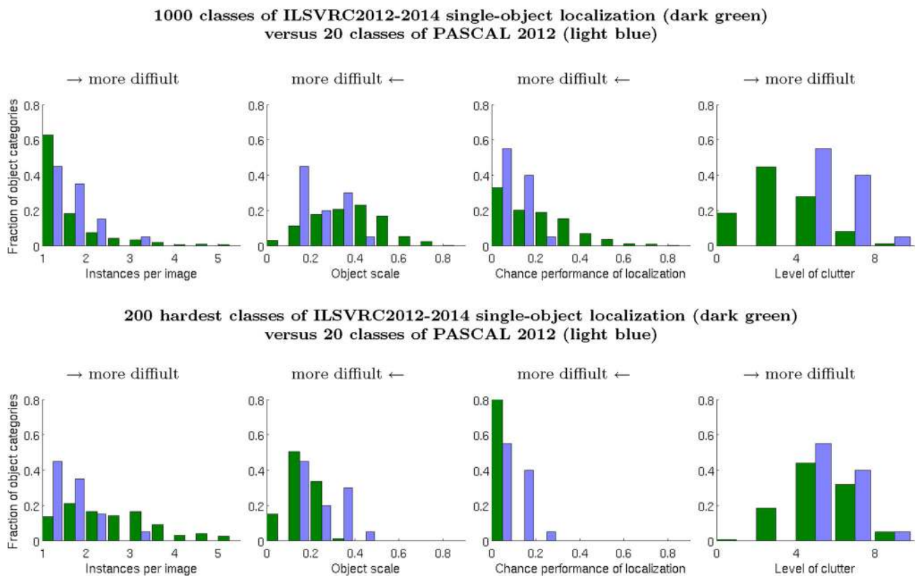
Fig. 16 Distribution of various measures of localization difficulty on the ILSVRC2012-2014 single-object localization (dark green) and PASCAL VOC 2012 (light blue) validation sets. Object scale is fraction of image area occupied by an average object instance. Chance performance of localization and level of clutter are defined in Appendix 1. The
