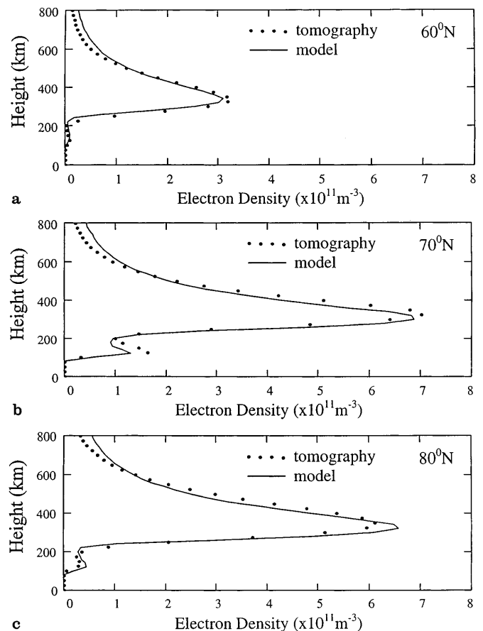
Fig. 4a–c. Comparisons of modelled ( solid lines ) and reconstructed ( dotted lines ) altitude profiles of electron density at latitudes of a 60°N, b 70°N and c 80°N
