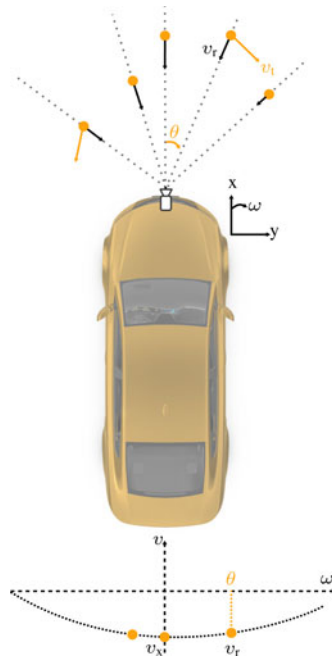
Fig. 3. Diagram clarifying the position of the radar and targets [18]. Target velocity ( v_t ) vectors are displayed in orange while the radial velocity ( v_r ) vectors in black. The coordinate system to the right of the car shows the orientation and direction of x , y , and \omega axes. In the bottom part of the figure, the velocities are plotted against the azimuth angle ( \omega ) for the stationary targets. v_x represents the ego velocity since it is in the same direction as the heading vector.
