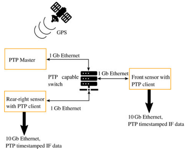
Fig. 6. PTP network architecture for accurate time synchronization between the front (calculate trajectory) and rear-right (SAR measurements) radar sensor.
