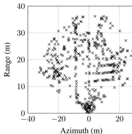
Fig. 9. Plot of detections obtained from output of the updated processing chain.
