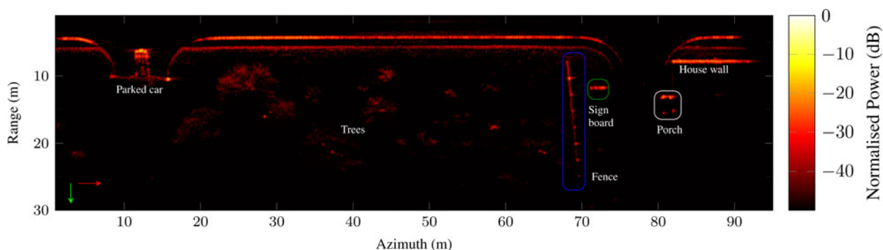
Fig. 18. Processed SAR image of scenario from Fig. 17. Trajectory start point is in the top left corner. Ego speed is 25 km/h.
