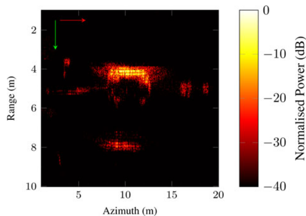
Fig. 15. Processed SAR image of scenario from Fig. 14. Trajectory start point is in the top left corner. Ego speed is 20 km/h.
