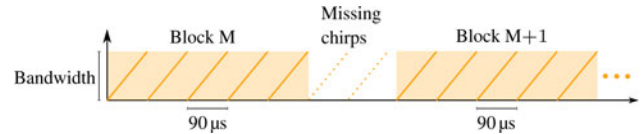
Fig. 11. Diagram illustrating how some chirps are missing between two blocks of chirp sequences.
