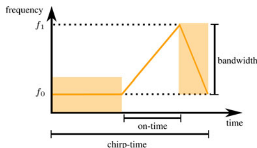
Fig. 2. Visual explanation of in-chirp duty cycle. f_0 denotes the start frequency.
