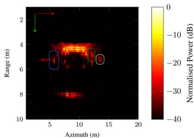
Fig. 13. Processed SAR image of scenario from Fig. 12. Trajectory start point is in the top left corner. Ego speed is 10 km/h.
