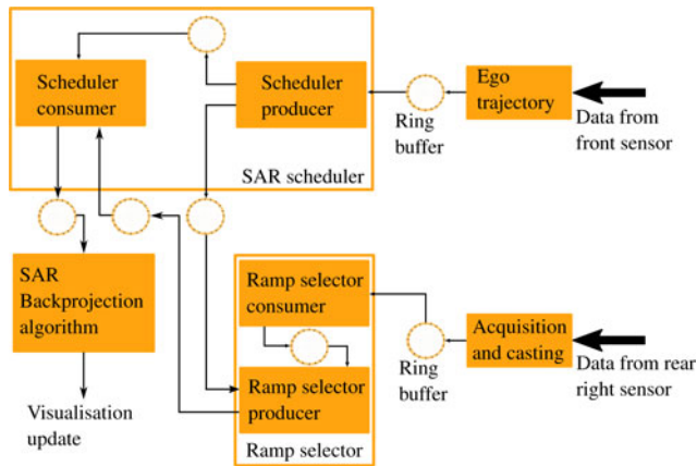
Fig. 10. Data flow diagram depicting how and where data from both the front and rear-right radar sensors are processed.
