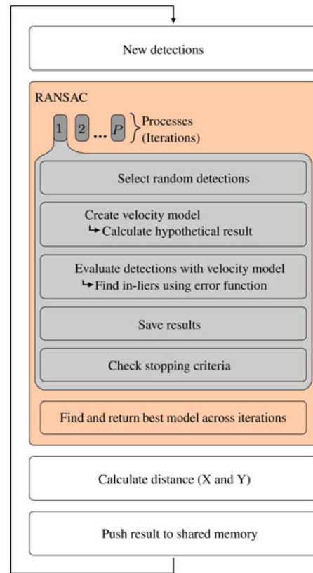
Fig. 5. Flow diagram depicting the processing steps for the ego trajectory calculation.
