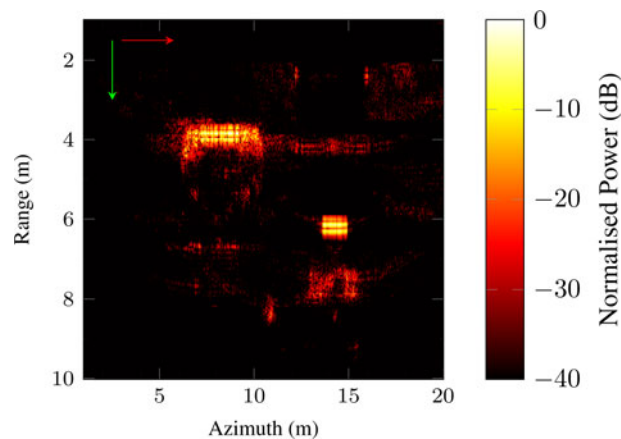
Fig. 16. SAR image of car parked next to a block of concrete. Trajectory start point is in the top left corner. Ego speed is 45 km/h.
