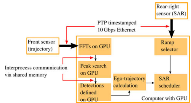
Fig. 7. Processing chain and data flow diagram showing detailed steps for the front sensor.
