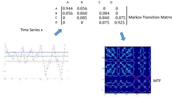
Figure 2: Illustration of the proposed encoding map of Markov Transition Fields. X is a sequence of time-series in the 'ECG' dataset. X is first discretized into Q quantile bins. Then we calculate its Markov Transition Matrix W and finally build its MTF with eq. (8).
